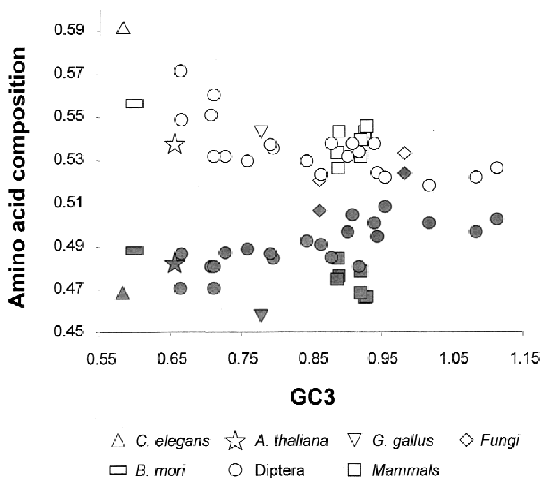
Fig. 2. Relationship between the frequencies of the high-GC (filled symbols) and low-GC (open symbols) amino acids and the frequency of GC content in third codon positions (GC3) for Xdh . Each data point in each group represents 1 of the 34 species studied. The GC frequencies are angularly transformed, so may reach values higher than 1.
