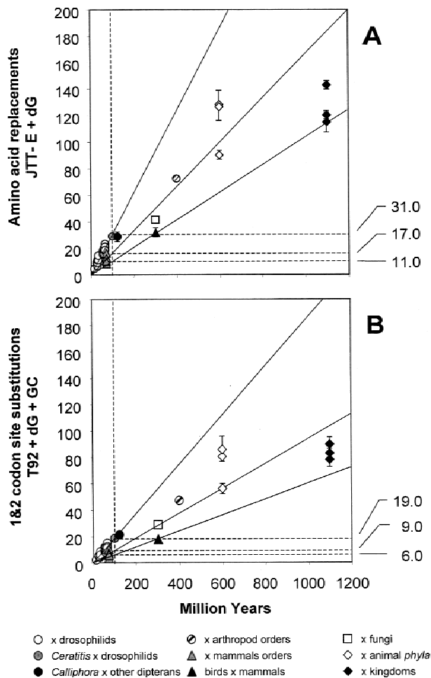
Fig. 5. Global rates of amino acid replacement for XDH (A) and nucleotide substitution rates in the first plus second codon positions as inferred with the T92 + dG + GC model (B). The rates on the right are replacements \times 10^{-10} per site per year; the rates correspond to the comparisons between the drosophilids (31.0 and 19.0 for A and B, respectively), between mammal orders (17.0 and 9.0), and between birds and mammals (11.0 and 6.0). The regressions are conducted as in Fig. 3, and the slopes are 0.0031, 0.0017, and 0.0011 for A and 0.0019, 0.0009, and 0.0006 for B. The amino acid replacement rate ( \times 10^{-10} per site per year) is 19.2 between animal phyla and 11.5 between the kingdoms; see Table 3 (regression lines are not shown).
