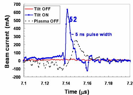
Figure 7: 52 fold neutralized compressed beam (blue line), non-neutralized compressed beam (dotted line) and non compressed beam current (red line) measured using pinhole Faraday cup.
