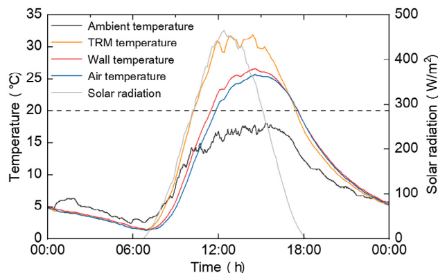
Fig. 10. The temperature variations of the SBED in heating mode on March 1, including ambient temperature (black curve), TRM temperature (orange curve), wall temperature (red curve) and air temperature (blue curve). Solar radiation intensity (grey curve) is given for reference.
