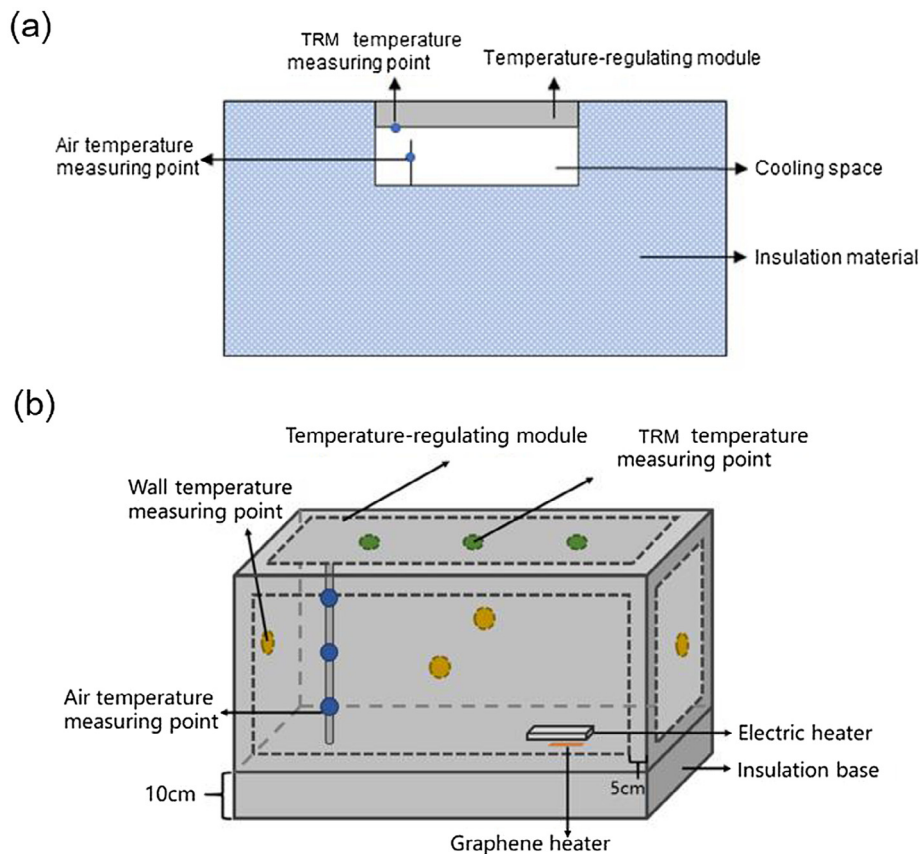
Fig. 2. Schematics of the experimental setup. (a) Schematic of the general radiative cooling experimental device (RCED). (b) Schematic of simulated building experimental device (SBED) with temperature measurement points and electric heater.
