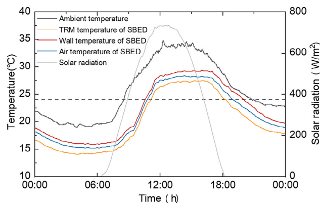
Fig. 6. The temperature variations with time in the SBED on February 15, including ambient temperature (black curve), TRM temperature (orange curve), wall temperature (red curve) and air temperature (blue curve). Solar radiation intensity (grey curve) is given for reference.
