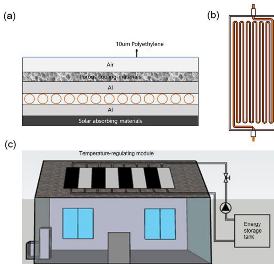
Fig. 20. Combination of the TRM and energy storage system. (a) Cross-section of the TRM with the coil. (b) Schematic of the combination of the TRM and the coil. (c) Schematic of the building employing the TRM with energy storage system.
