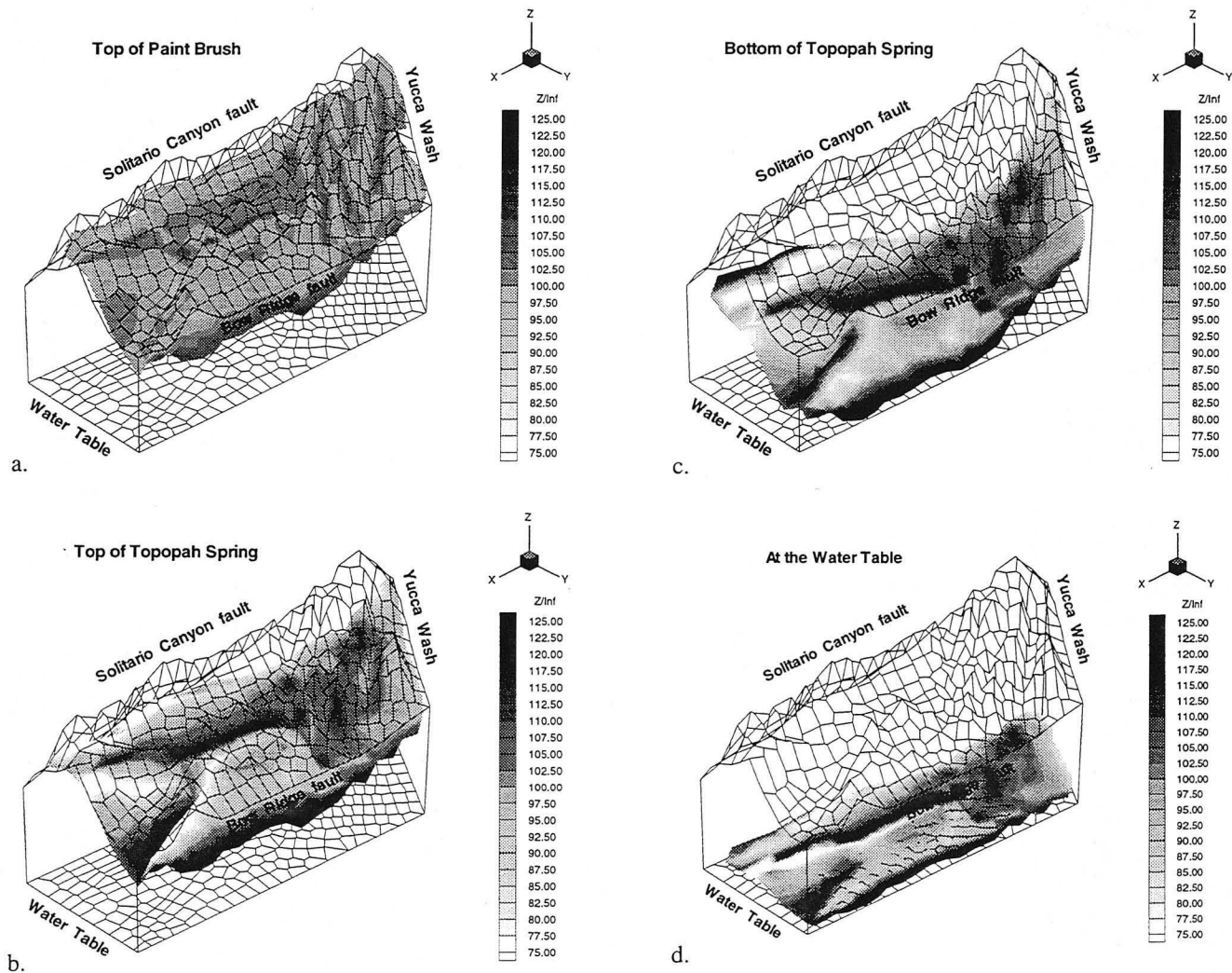
Figure 4. Calculated normalized vertical moisture fluxes (% of infiltration at ground surface) at different depths in the site-scale model for the case of “capillary barrier” faults, and an uniform areal infiltration rate of 0.1 mm/year.
