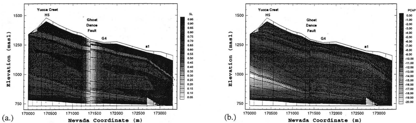
Figure 2. Two-dimensional cross section S-S' showing calculated distributions of liquid saturation (2a) and capillary pressure (2b).
