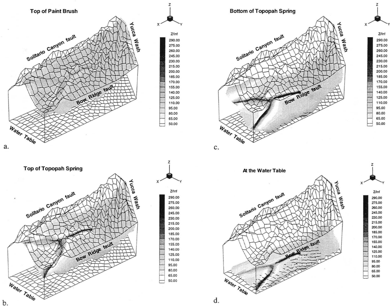
Figure 5. Calculated normalized vertical moisture fluxes (% of infiltration at ground surface) at different depths in the site-scale model for the case of “permeable” faults, and an uniform areal infiltration rate of 0.1 mm/year.
