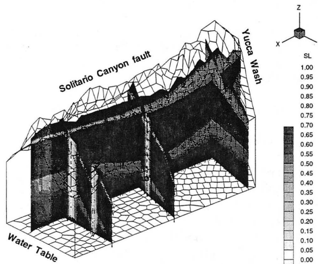
Figure 3. A quasi-three-dimensional calculated liquid saturation at Yucca Mountain shown using data for cross sections R-R', S-S', T-T' and V-V' (see Figure 1)
