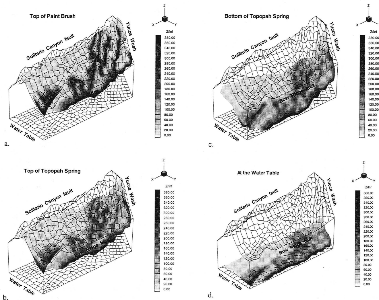
Figure 6. Calculated normalized vertical moisture fluxes (% of average net infiltration) at different depths in the site-scale model for the case of “capillary barrier” faults, and non-uniform infiltration (average 0.1 mm/year).
