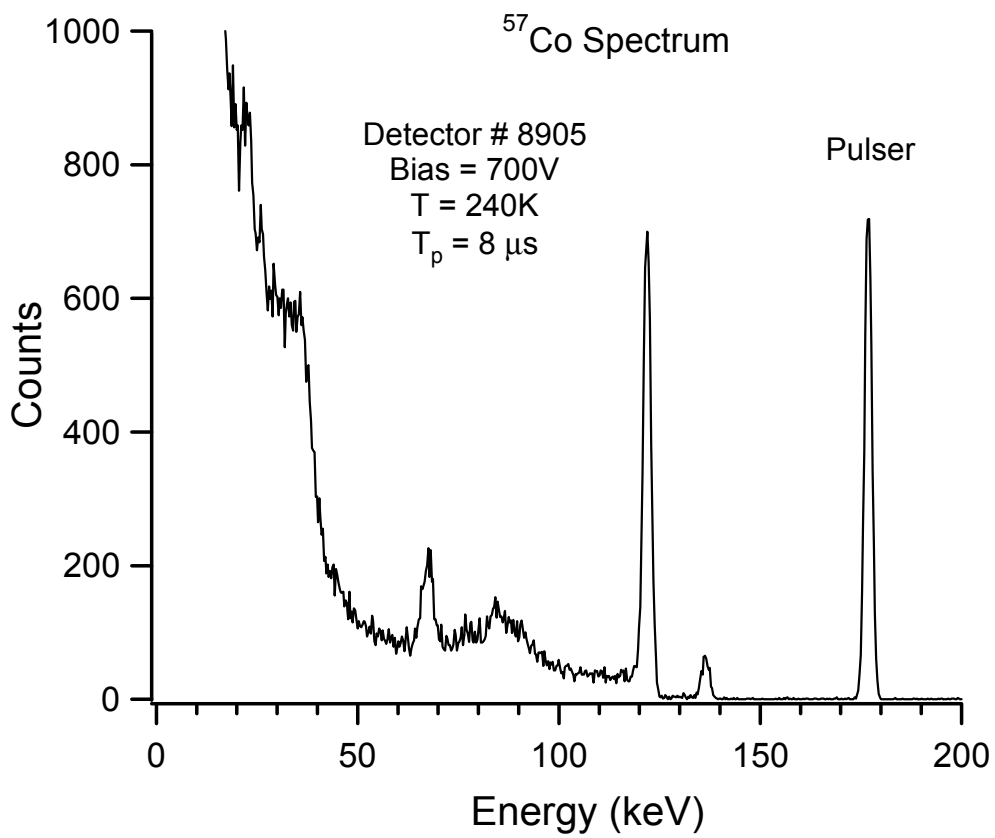
Figure 6 - A spectrum of ^{57}\text{Co} taken using a 6mm thick Si(Li) detector operating at 240K, 700V bias and T_p = 8 \mu\text{s} . The FWHM of the 122 keV peak is 2.1 keV.
