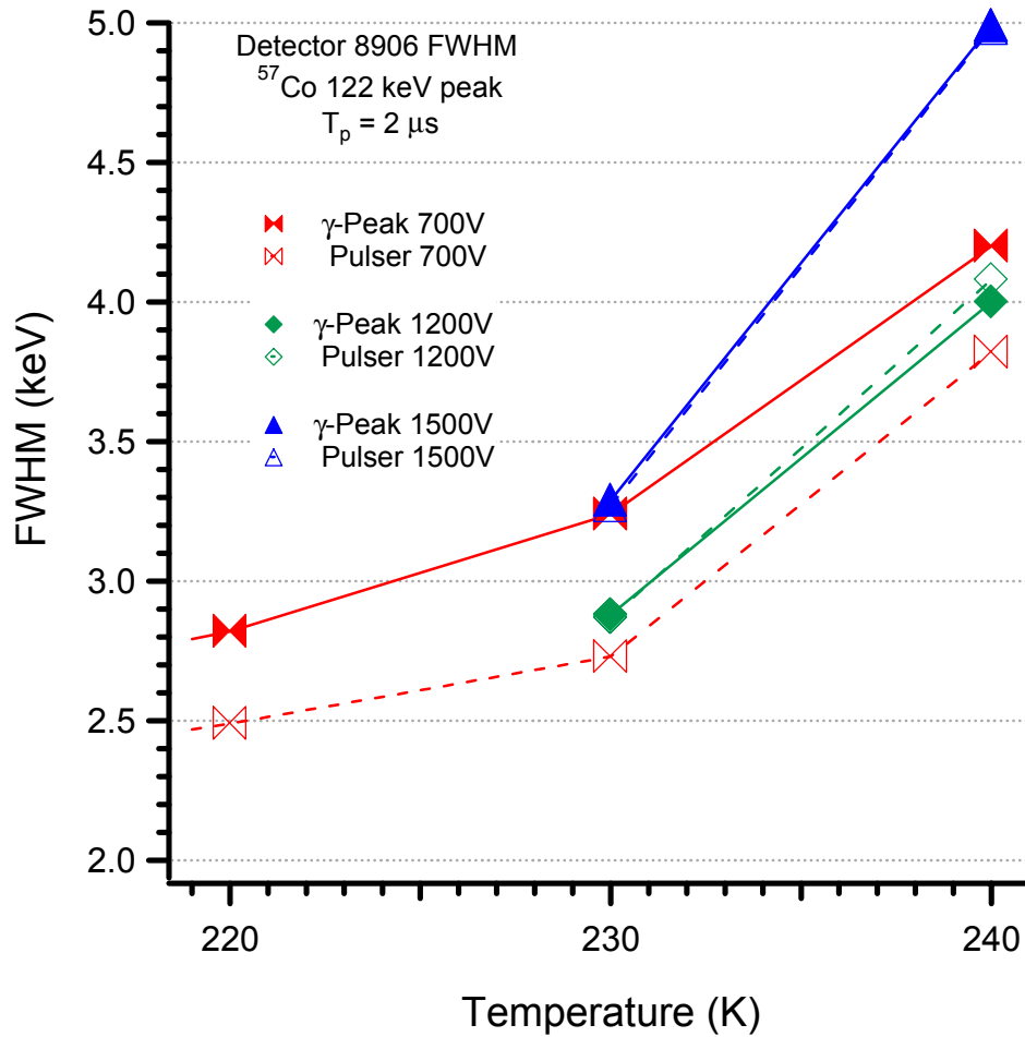
Figure 8 - Width of the ^{57}\text{Co} 122 keV peak vs. temperature at three different bias voltages, compared with the electronic noise for a Si(Li) detector with a deep groove but no guard ring.
