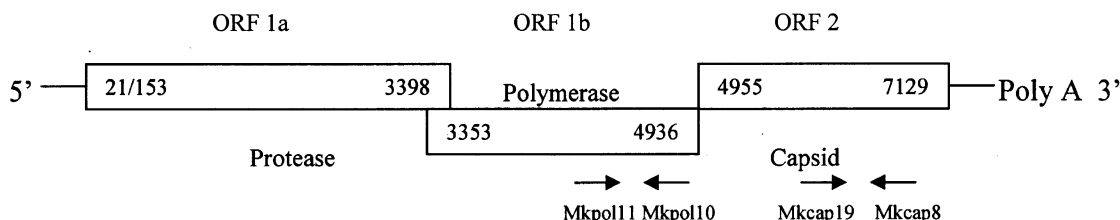
Fig. 1 Diagram of the turkey astrovirus genomic organization and location of primers used for amplification of segments of the polymerase and capsid genes. Numbers within the diagram represent the predicted start and stop sites. Primer sites are indicated with arrows
