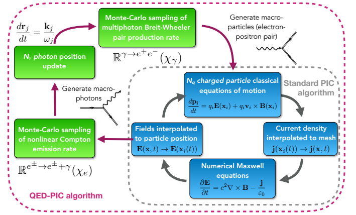
FIG. 6. Framework of QED PIC.
