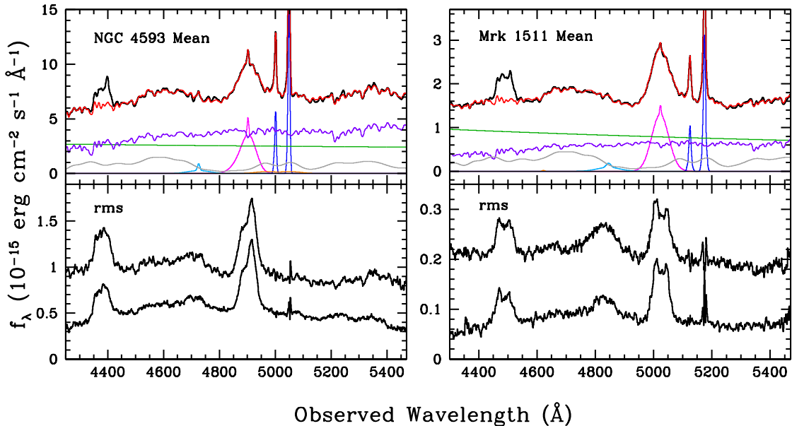
FIG. 3.— Same as Figure 2, but for fits done using the Boroson & Green (1992) Fe II template.
