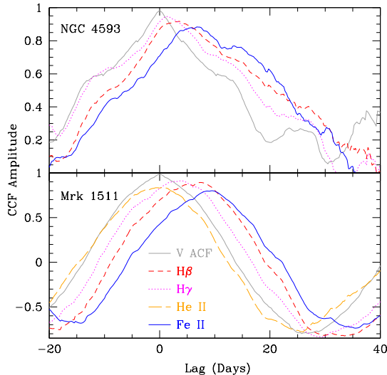
FIG. 4.— Cross-correlation functions for H\beta , H\gamma , He II, and Fe II relative to the V-band photometric light curves. The autocorrelation function of the V-band light curve is shown in grey.
