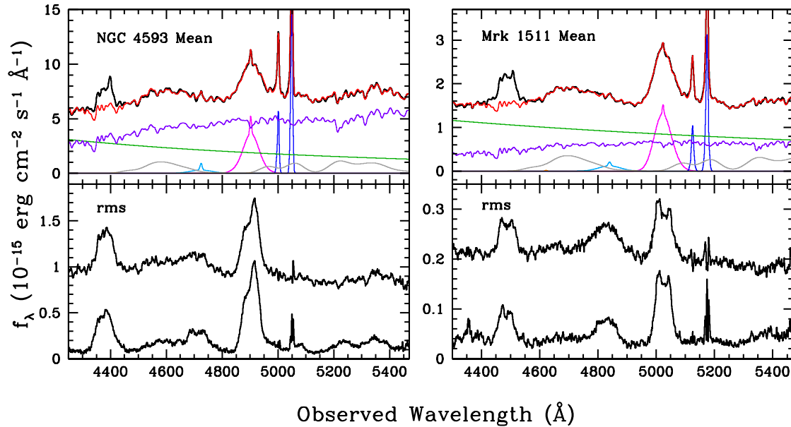
FIG. 6.— Same as Figure 2, but for fits done using the Kovačević et al. (2010) Fe II templates. The grey curve represents the sum of the five individual Fe II components.
