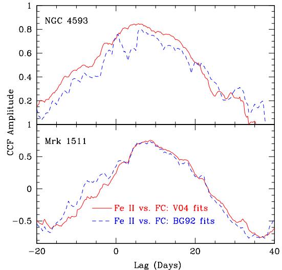
FIG. 5.— Cross-correlation functions for Fe II relative to the AGN featureless continuum (FC) measured from the spectral fits done using the BG92 and V04 Fe II templates.
