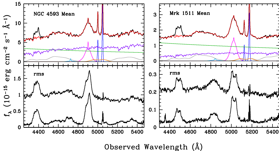
FIG. 2.— Mean and rms spectra of Mrk 1511 and NGC 4593. Upper panels: Mean spectrum (black) overlaid with the model fit done using the Véron-Cetty et al. (2004) Fe II template (red). Individual fit components include the AGN power law (green), old stellar population (purple), Fe II emission (grey), H \beta (magenta), [O III] (blue), He II (light blue), and He I (orange). Lower panels: The standard rms spectrum (top) and an rms spectrum constructed from individual nightly spectra after the AGN power-law and stellar components were removed (bottom).
