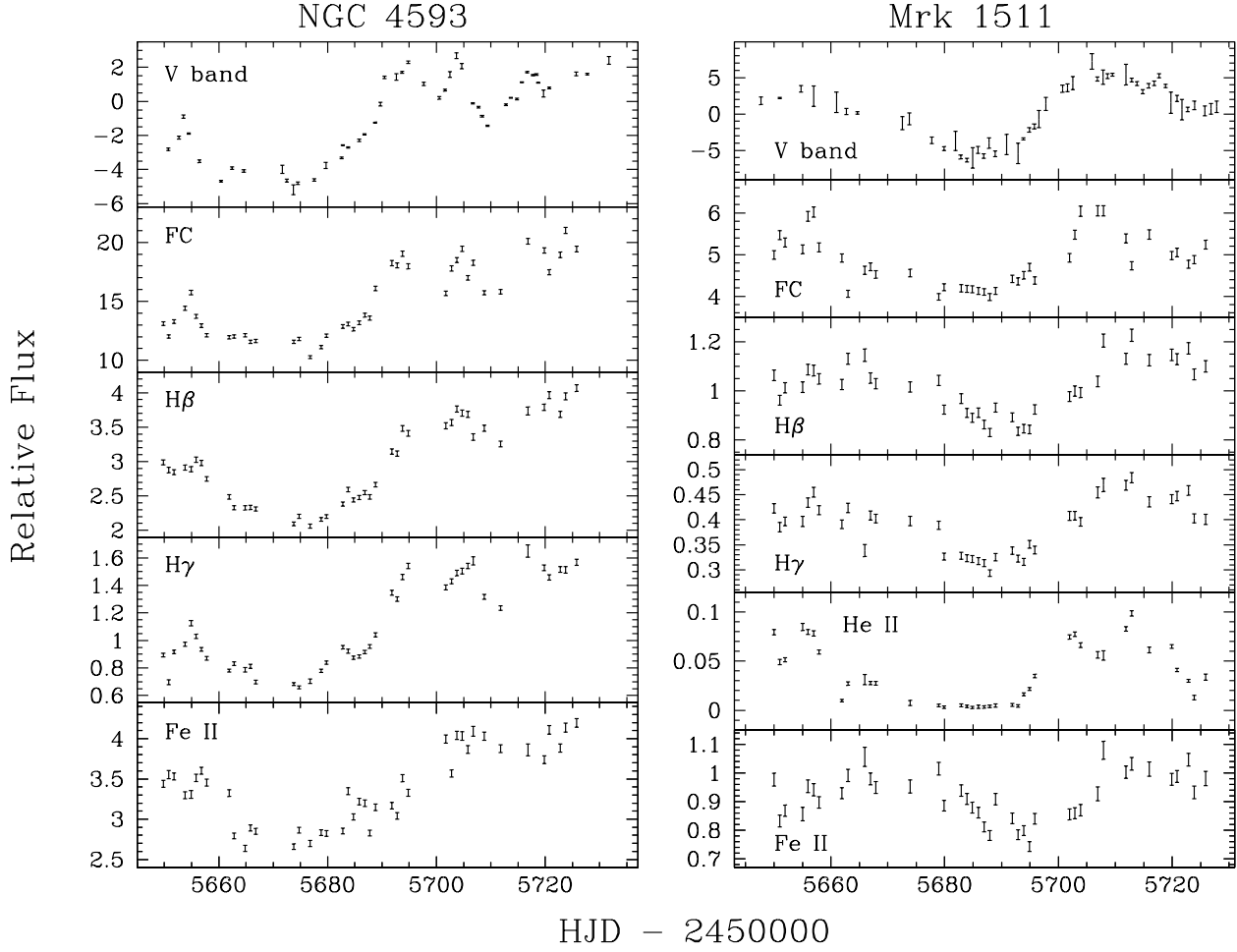
FIG. 1.— Light curves of the V band, the AGN featureless continuum (FC), H \beta , H \gamma , He II (for Mrk 1511 only), and Fe II. The Balmer-line and He II light curves contain flux from narrow components, including [O III] \lambda 4363 in the H \gamma light curve. The V-band photometric light curves are given in differential flux units (i.e., relative to the flux in a reference image), as determined by the image-subtraction photometry procedure. The FC and emission-line light curves are those measured from the spectral fits which used the Véron-Cetty et al. (2004) Fe II template.
