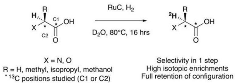
Scheme 1: Regioselective catalytic deuterium labelling via 1H/2H exchange using ruthenium on carbon (RuC).
