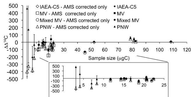
Figure 4. \Delta^{14}\text{C} values of processed samples minus those of bulk samples ( \Delta^{14}\text{C} corrected for C_{\text{ex}} ) from ^{14}\text{C} -modern or near modern and subfossil samples. Open symbols are corrected for combustion, graphitization, and graphite target handling only ( C_{\text{AMS}} ), and filled symbols are corrected for C_{\text{chemistry}} and/or C_{\text{HPLC}} as well as C_{\text{AMS}} . All data were corrected for isotopic fractionation with online \delta^{13}\text{C} -AMS values as stated in the text. Samples containing <2 \mu\text{gC} are plotted here and shown in italics in Tables S-1 and S-2 (Supporting Information) for illustration only. The \Delta^{14}\text{C} values of these samples are not meaningful because the mass of the total blank correction applied is bigger than the mass of the samples, as mentioned in the text.
