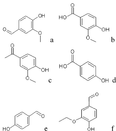
Figure 1. Structures of lignin phenols that were purified for radiocarbon analysis including (a) vanillin, (b) vanillic acid, (c) acetovanillone, (d) 4-hydroxybenzoic acid, (e) 4-hydroxybenzaldehyde, and (f) ethyl vanillin.
