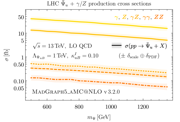
FIGURE 4: Cross sections of \bar{\Psi}_u single production in association with up to two photons and/or Z bosons. Cross sections for \Psi_u and \bar{\Psi}_d , \bar{\Psi}_d are smaller in analogy with single production ( viz. Figure 2 and discussion).
