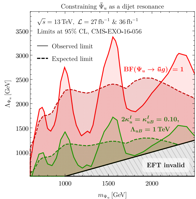
FIGURE 6: Parameter space excluded for sextet antifermion coupling to up-type quarks ( \bar{\Psi}_u ) based on a CMS dijet resonance search at \sqrt{s} = 13 \text{ TeV} . All limits are computed assuming \sigma(pp \rightarrow \bar{\Psi}_u) as displayed in Figure 3; but red regions assume unit branching fraction to \bar{u}g , while green regions take more realistic branching fractions of around 26%. In the gray region, where m_{\Psi_u} > 2\Lambda_{\Psi_u} , the EFT is unlikely to be consistent.
