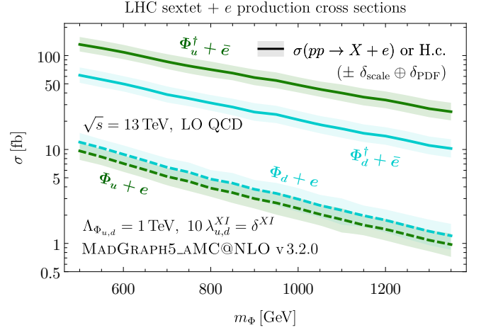
FIGURE 5: Cross sections of sextet scalar single production in association with an electron or positron. Conjugate scalar production dominates in a fashion similar to sextet fermion single production. Cross sections for associated production with \mu, \tau are orders of magnitude smaller if all else is equal.
