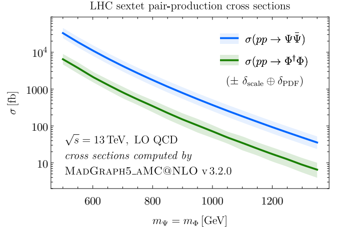
FIGURE 2: Leading order cross sections for pair production of color-sextet fermions and scalars at the LHC as a function of sextet mass.
