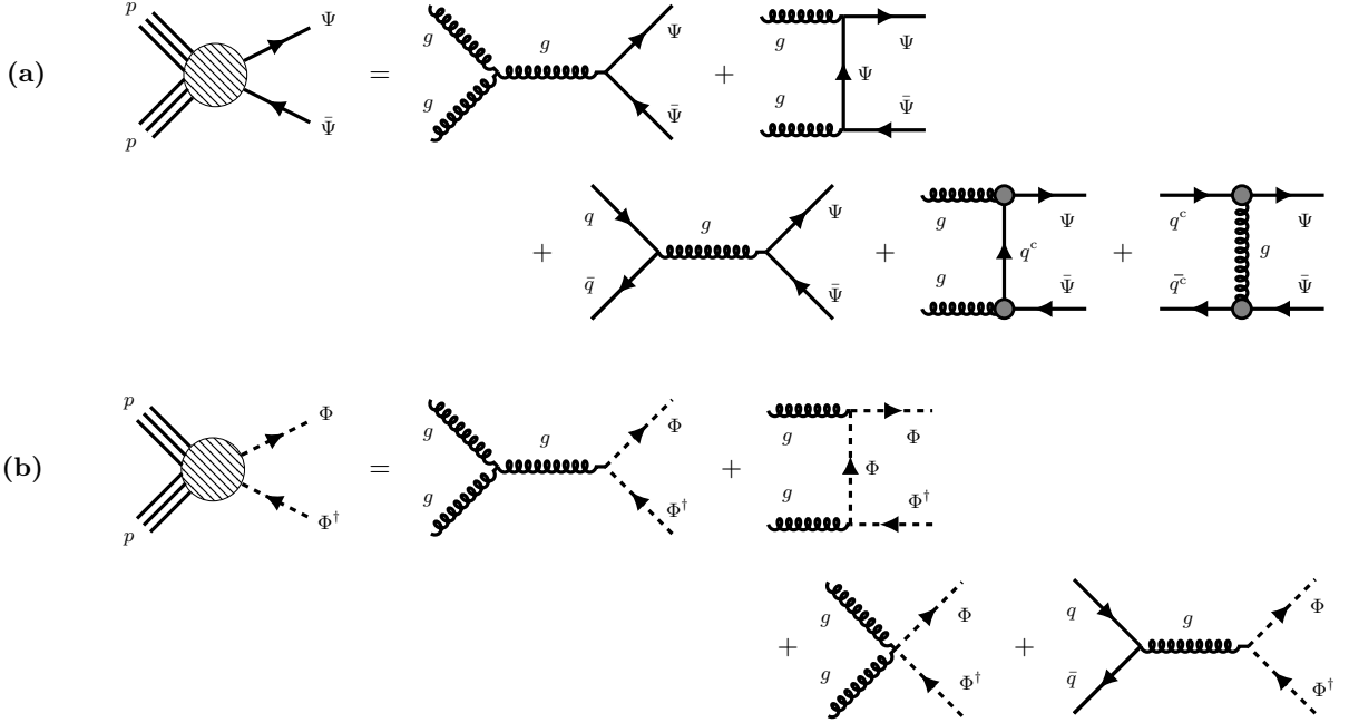
FIGURE 1: Representative diagrams for pair production of color-sextet (a) fermions and (b) scalars. Blobs mark vertices corresponding to an effective operator with some cutoff scale. Quarks coupling directly to sextets must have appropriate hypercharge; viz. (12) and (13). These contributions are negligible for realistic \Lambda_{\Psi_u}, \Lambda_{\Psi_d} .
