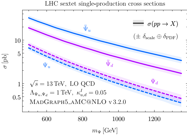
FIGURE 3: Cross sections of color-sextet fermion single production. These are comparable to fermion pair-production cross sections for indicated couplings/cutoffs. Conjugate fermion ( \bar{\Psi} ) cross sections dominate because quarks have greater parton luminosity than antiquarks at LHC.
