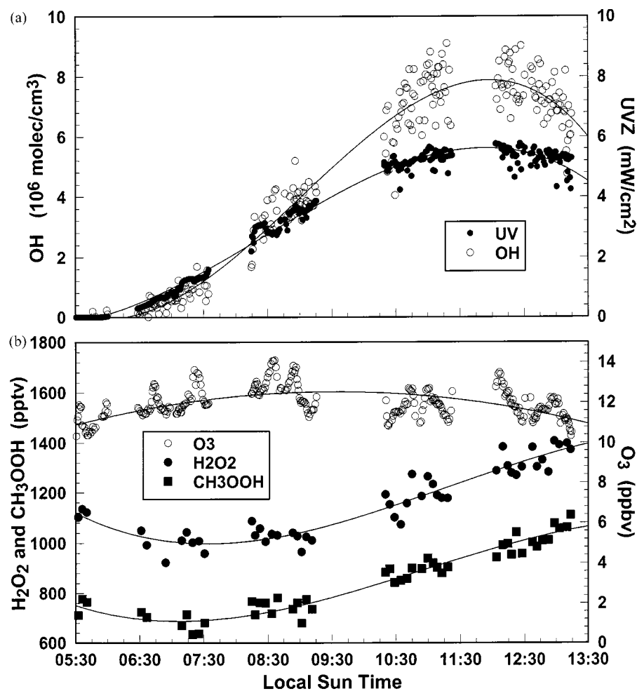
Figure 1. Time series plots for (a) OH and UVZ and (b) \text{O}_3 , \text{H}_2\text{O}_2 and \text{CH}_3\text{OOH} . Trend lines shown represent polynomial fit. Data recorded in the vicinity of Christmas Island on August 24th, 1996.
