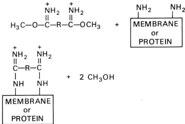
Fig. 1. Amidination reaction.
