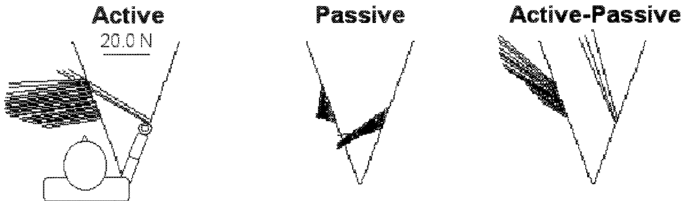
Figure 5. Example of assessment of incoordination. Data is from a female, chronic hemiparetic, traumatic brain-injured subject. Subject reached at a comfortable speed ten times as far as possible, or underwent four slow passive movements with the arm relaxed, with the ARM Guide locked in two orientations (yaw=22.5, elevation=+30). Shown is the top view of the forces generated during active and passive movement. Active: The force difference between the impaired and unimpaired arms during active reaching at matched speeds. Note that the impaired arm differentially generates a large, medially directed force in both ARM Guide orientations, consistent with the abnormal extension synergy. Passive: The difference between impaired and unimpaired arms during slow, imposed movement with the subject relaxed. Note that the impaired arm prefers a more internally rotated, flexed posture, resisting movement outward along the guide. Active-Passive: The difference between active and passive movement for the impaired arm. Note the impaired directional force control, due to active contraction of muscles.
