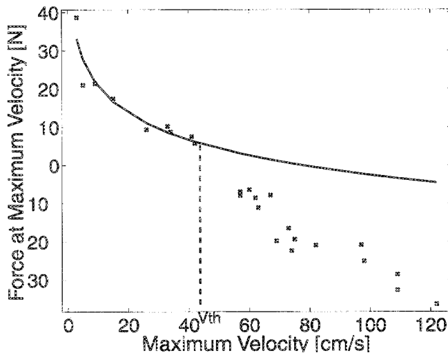
Figure 4. Force-velocity profile for a chronic stroke subject. The solid curve represents a negative power fit to the data before the threshold velocity ( V_{th} ) to approximate the Hill force-velocity relationship. The dotted line demarcates where the data skew from the Hill relationship, signifying activation of spastic stretch reflexes resisting movement.
