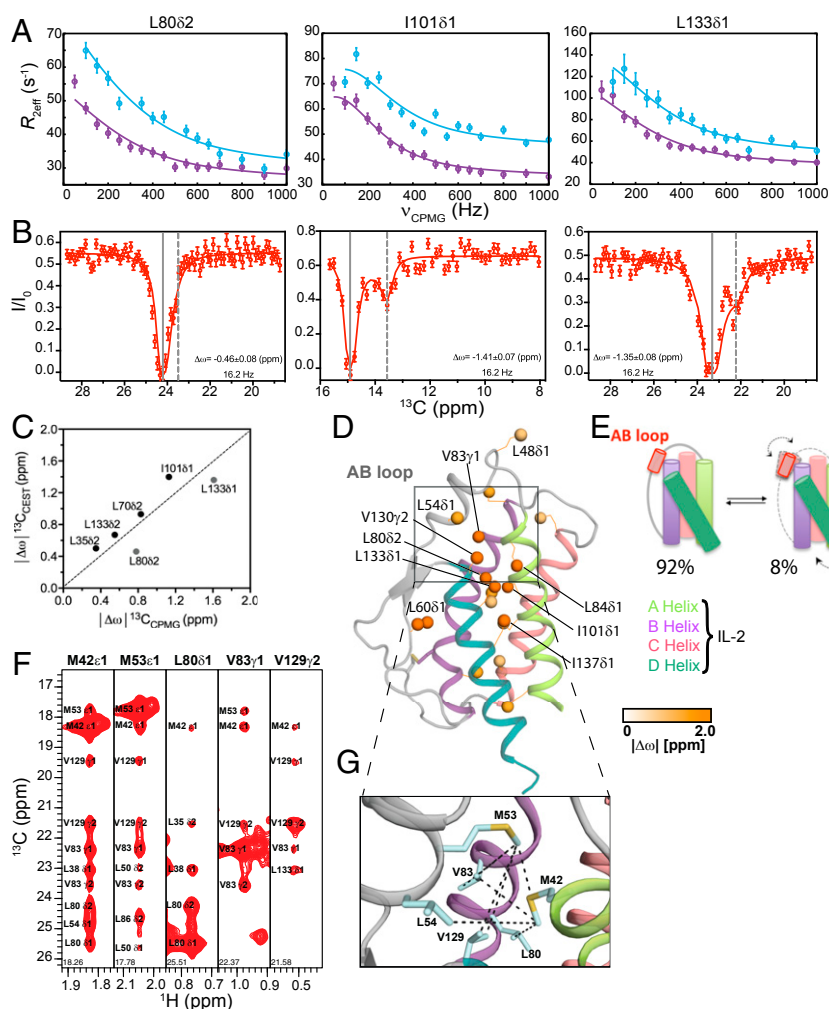
Fig. 2. Solution dynamics and ground-state structure of free mIL-2 by methyl NMR. (A) Methyl-selective ^{13}\text{C} single quantum CPMG relaxation dispersion profiles carried out at two magnetic fields (600 MHz, purple; 800 MHz, blue) are shown for selected residues in the B helix (L80 \delta_2 ), C helix (I101 \delta_1 ), and D helix (L133 \delta_1 ) of WT free mIL-2. Experimental data are shown as small circles in all panels, with errors estimated from the S/N in the raw experimental data. The best-fit lines are shown for a global analysis of 20 methyls with nonflat relaxation dispersion profiles using a two-site conformational exchange model. (B) ^{13}\text{C} -CEST profiles carried out at 800 MHz for L80 \delta_2 , I101 \delta_1 , and L133 \delta_1 . Plots of normalized intensity of the ground state resonance relative to a control experiment where the saturating field is highly off-resonance (12 kHz), as a function of the position of the perturbing B_1 field (with a measured strength of 16.2 Hz). Uncertainties in the normalized intensity ( I/I_0 ) are determined from the root-mean-square deviation in the baseline of the raw CEST profiles where no intensity dips are present (typically, n > 30 ). Global fits of the CEST data to a two-site model of chemical exchange are shown as solid red lines. The resonances of the major state (gray solid lines) and fitted minor state (gray dashed lines) are indicated, with the resulting chemical shift difference shown in each plot. (C) Linear correlation plot of chemical shifts of the excited state of WT mIL-2 obtained from ^{13}\text{C} CPMG (x axis) and ^{13}\text{C} CEST (y axis). CPMG and CEST experiments were recorded at 25 °C and 10 °C, respectively. (D) Twenty methyl probes undergoing chemical exchange by CPMG are shown as spheres on the model structure of mIL-2 and colored orange according to the magnitude of fitted |\Delta\omega| values. (E) Schematic representation of mIL-2 illustrating the interconversion between a ground state, which is 92% populated, and an invisible, excited state, which is ~8% populated. The dotted arrows represent the coupled conformational transition of the AB loop and the hydrophobic core of mIL-2. (F) ^{13}\text{C}_\text{M}-^1\text{H}_\text{M} strips from a 3D \text{C}_\text{M}-\text{C}_\text{M}\text{H}_\text{M} SOFAST NOESY experiment taken at the ^{13}\text{C}_\text{M} coordinates of stereospecifically assigned methyl resonances noted on each panel, showing NOE cross-peaks between the methyl resonances of residues on the AB Loop. (G) Close-up view of the AB loop region from a Rosetta homology-based model of free mIL-2 (using PDB ID 1M47 as a template) showing the network of observed NOEs (black dotted lines), corresponding to the major (ground-state) solution conformation. The pattern of NOEs is consistent with a “closed” conformation of free mIL-2, with where the AB loop is well-packed against the hydrophobic core of the structure.
