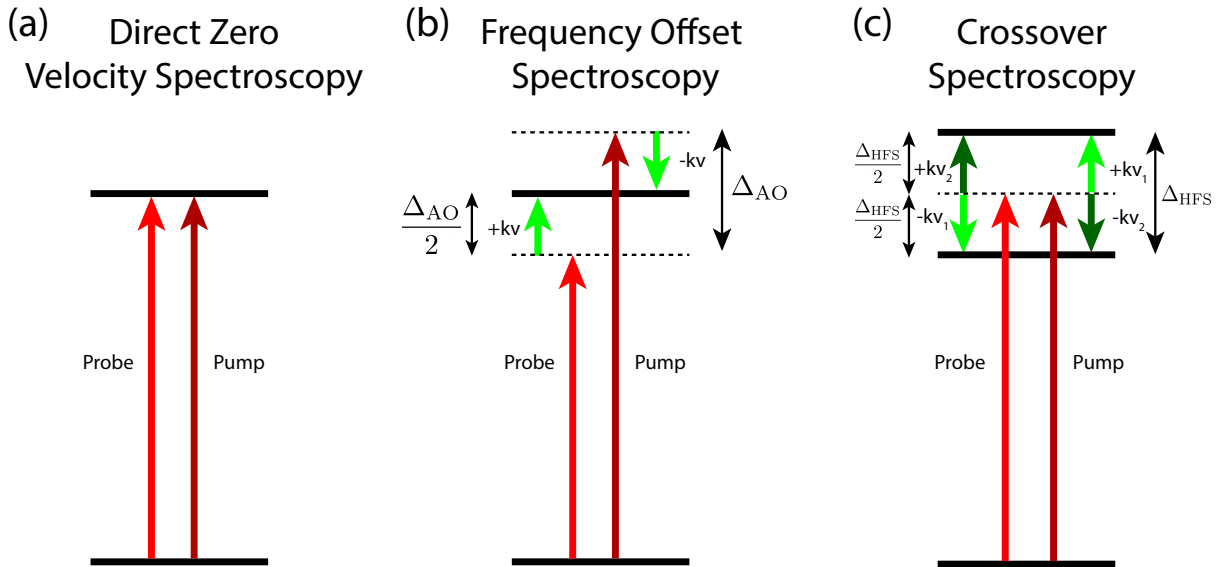
Figure 2.5: Saturated absorption spectroscopy techniques. (a) In direct saturated absorption spectroscopy, atoms moving with zero velocity are optically excited by the pump beam so that the probe experiences less absorption as it propagates through the medium than it would in the absence of the pump. This creates a sub-Doppler feature in the probe spectroscopy signal to which a laser can be locked. (b) In frequency offset spectroscopy, the pump and the probe are detuned by \Delta_{AO} from each other so that they are never simultaneously resonant with any transition. However, when the probe is red detuned by -\Delta_{AO}/2 from a transition then the pump is blue detuned by \Delta_{AO}/2 . There is, then, a certain subset of atoms moving towards the probe with velocity v such that the Doppler shift kv = \Delta_{AO}/2 blue (red) detunes the probe (pump) onto resonance. (c) In the simplest form of crossover spectroscopy, the pump and the probe are at the same frequencies and detuned halfway between two atomic transitions. There is, then, a class of atoms whose Doppler shift red or blue detunes the pump into resonance with one transition and blue or red detunes the probe onto resonance with another transition. A saturated absorption feature again appears in the probe spectroscopy signal because of the depletion of the ground state by the pump. Crossover spectroscopy can also be performed with the pump and probe detuned from each other if the pump and probe are also respectively detuned from two different transitions by equal and opposite amounts.
