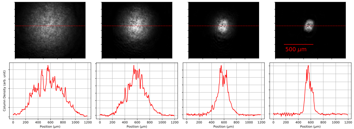
Figure 2.10: TOF images of atomic gas at various stages during the final optical evaporation. Evaporation proceeds from left to right. Notice the bimodal distribution apparent in the third panel and the complete disappearance of the thermal background in the fourth panel.
