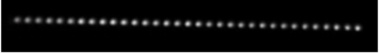
Figure 7.2: (33x) focused laser spots generated by imaging the AOD output using the high-NA objective. Here we see some variation in the intensity of the the different tweezer spots. In an experiment this intensity variation would need to be calibrated out and compensated for.
