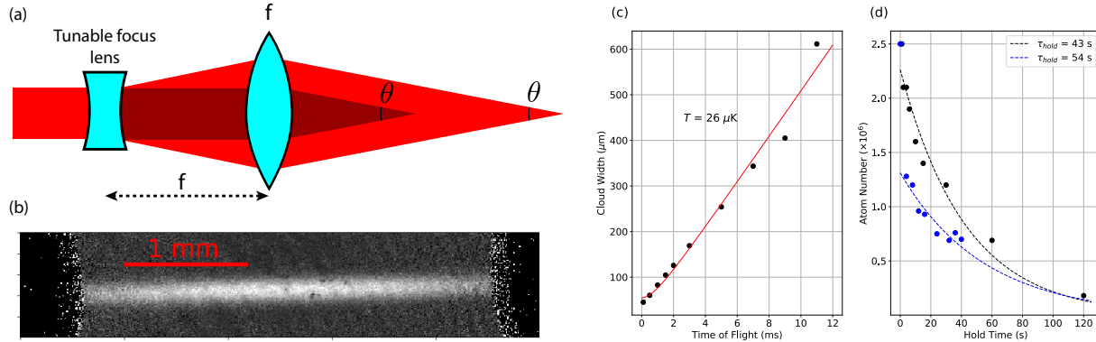
Figure 2.9: (a) We utilize a scheme described in Ref. [102] for optical transport. If the focal length of the tunable focus lens is adjusted, then the position of the focused waist will translate but the size of the waist will remain unchanged. (b) Absorption image of atoms released from the transport ODT after 500 \mu\text{s} of TOF. This image is taken perpendicular to the transport ODT axis and at 45^\circ to the science cavity, the mirrors of which can be seen as dark regions at the left and right sides of the frame. See Fig. 5.1(a). (c) TOF measurement of the temperature of the atoms in the transport ODT after transport. (d) Lifetime of atoms in the transport ODT while holding the atoms still and while continuously transporting the atoms.
