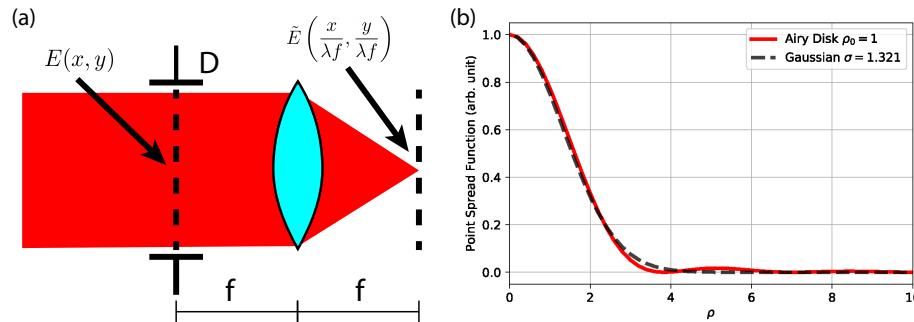
Figure B.1: (a) Fourier imaging schematic. A beam with profile E(x, y) impinges from the left passing through an iris of diameter D is focused by a lens with focal length f . In the paraxial limit, the spatial profile on the output plane is proportional to a scaled version of the Fourier transform of the input profile at the iris: \tilde{E}\left(\frac{x}{\lambda f}, \frac{y}{\lambda f}\right) . (b) Airy disk point spread function with scale factor \rho_0 (red) and Gaussian fit to this Airy disk (black). The best fit yields \sigma = 1.321\rho_0 .
