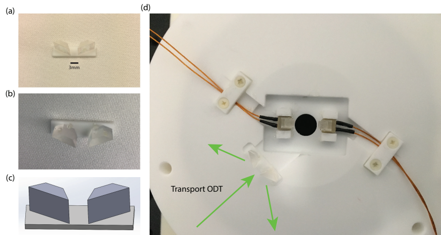
Figure 5.6: Photographs of the cavity shielding mirrors. Each mirrors is constructed from a piece of a small glass prism, one side of which has been coated with a reflection coating. The shielding mirrors were epoxied using UV-curing epoxy onto a shielding mirror plate. the angle was set by eye with reference to stencil. (a) photograph of the shielding mirrors after being epoxied. (b) Photograph of backside of shielding mirrors with drops of UV-curing epoxy visible. (c) CAD image of shielding mirrors on shielding mirror platform. (d) Image of shielding mirrors and cavity mirror assemblies on completed science platform. The shielding mirror plate is epoxied into a rectangular depression on the top of the science platform.
