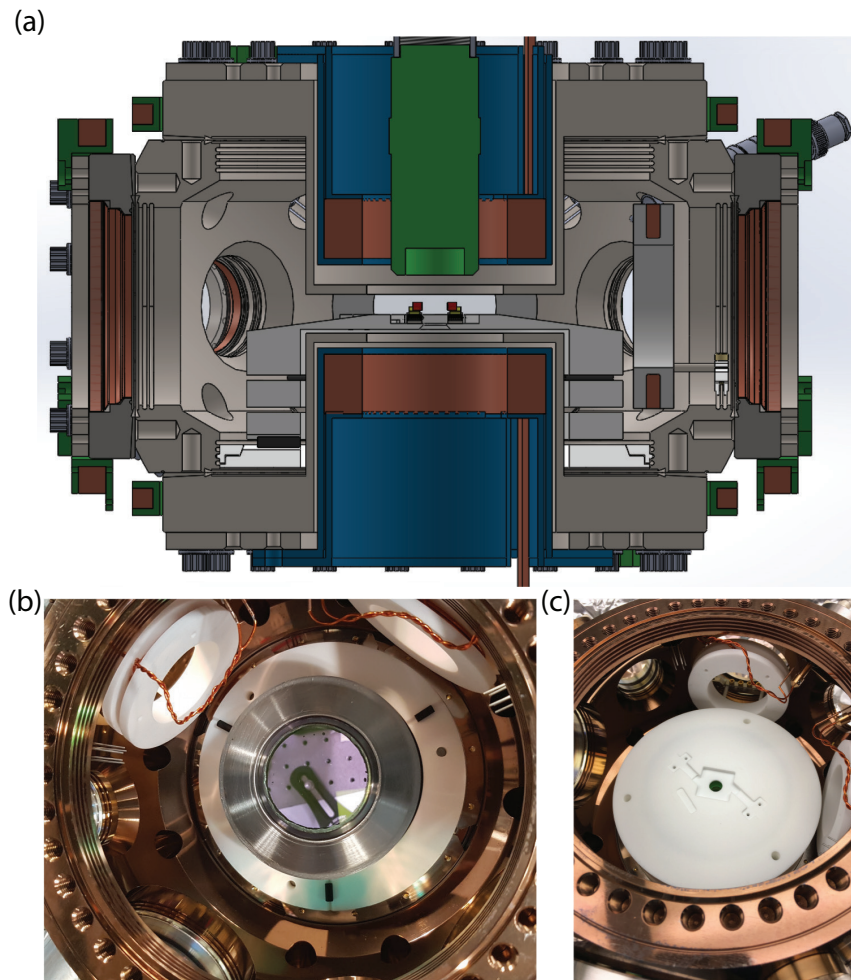
Figure 5.4: (a) Section view of CAD drawing of vibration isolation structure. Re-entrant viewport seen at center, three Macor vibration isolation stages (gray), some Viton cylinders (black), and groove grabber plate (white). Also seen are the cavity mirrors (red), the microscope objective (green), the anti-Helmholtz coils (copper), and the anti-Helmholtz coil clamps (Blue). (b) Image of science chamber after installation of first vibration isolation stage. (3x) black Viton cylinders can be seen. (c) Image of the bare science platform atop the vibration isolation system early in the chamber assembly process.
