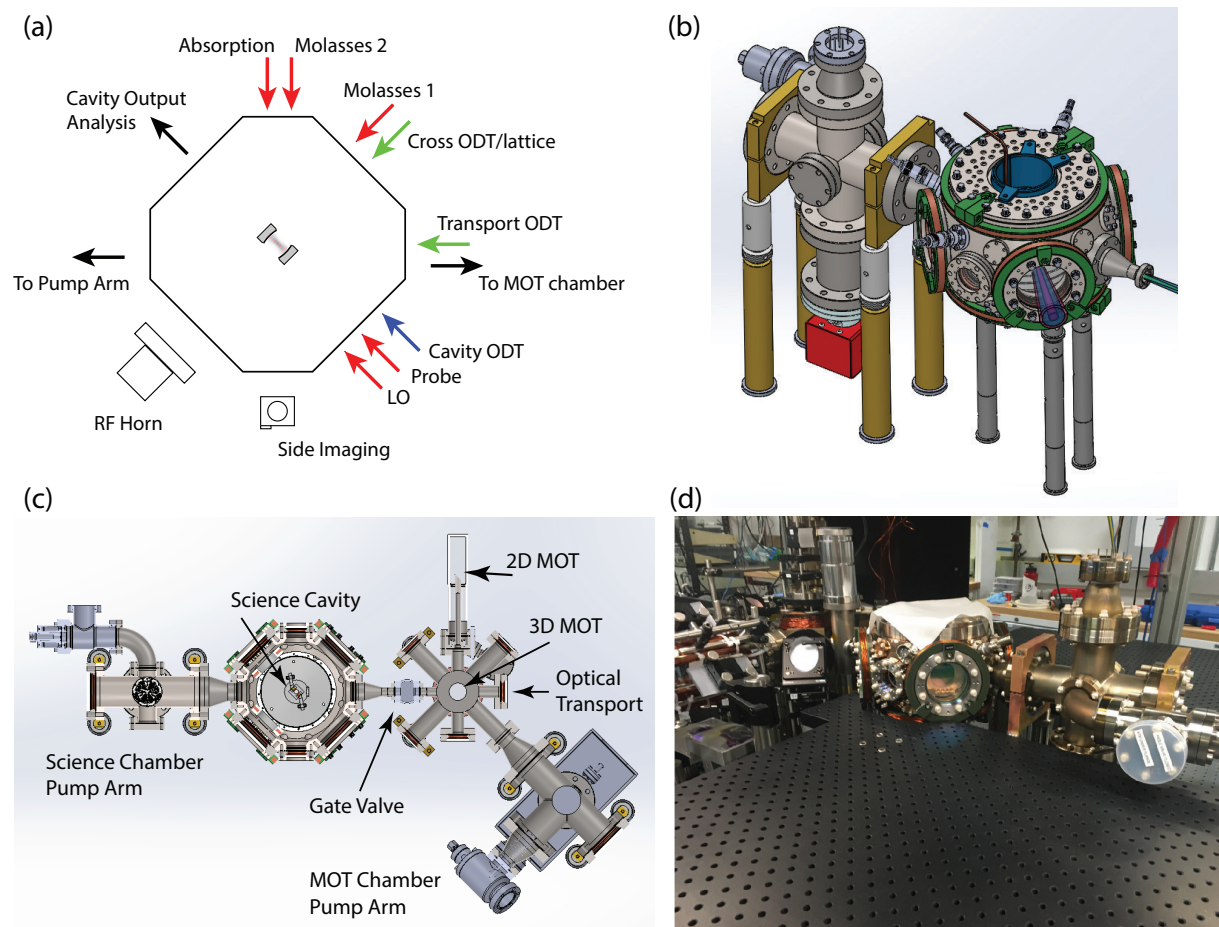
Figure 5.1: Overview of the science chamber. (a) Schematic diagram for the usage of each of the horizontal vacuum ports on the science chamber. Note that the science cavity is at 45^\circ to the transport axis. I will refer to the following axes throughout this text: The transport axis, the cavity axis, the vertical axis, the cross axis, and the absorption or side-imaging axis. (b) CAD image of the science chamber and science chamber pump arm. (c) CAD section view of the entire vacuum system. Atoms are collected in the 2D MOT where they are fired into the 3D MOT where they are cooled, optically trapped, and then optically transported into the science chamber. (d) Photograph of the science chamber and science chamber pump arm shortly after the vacuum bakeout and before the installation of many optics.
