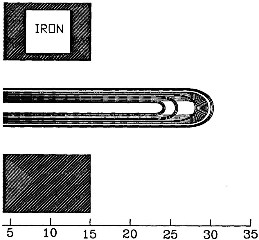
Figure 10 Coil and IRON in the end region of the SSC quad.
