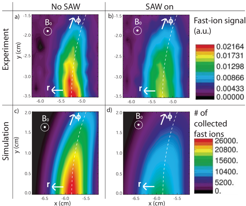
FIG. 1. (Color online) Comparison of Monte Carlo model simulated fast-ion beam profiles with experimental data. Contours in the same row use same color bar on the right for scaling. (Experimental orbit center is NOT LAPD center.)
