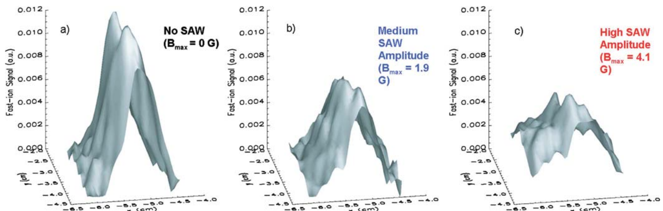
FIG. 4. (Color online) Comparison of fast-ion beam profile with different SAW amplitude. The z axis is fast-ion signal strength. (a) SAW antenna off. (b) Medium SAW amplitude ( B_{\max} = 1.9 G); (c) High SAW amplitude ( B_{\max} = 4.1 G). (Data were acquired with 100 MHz sampling rate, averaging eight samples and ten consecutive plasma shots, August 2008 LAPD run.)
