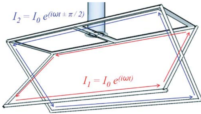
FIG. 3. (Color online) Illustration of the quadruple current channel antenna.
