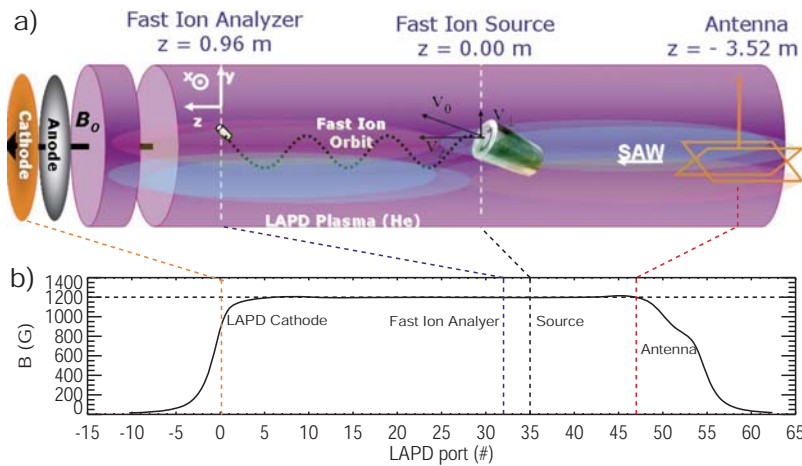
FIG. 2. (Color online) Experimental setup at the LAPD. (a) Overview of instruments (not to scale, dotted helix is the fast ion orbit; white box denotes the fast ion-SAW interaction region). (b) Ambient magnetic field profile vs LAPD port number (black solid). The distance between two adjacent ports is 0.32 m. Instruments' typical locations are marked by dashed perpendicular lines.
