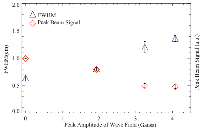
FIG. 5. (Color online) FWHM of the radial profile (triangle) and peak beam signal amplitude (diamond) vs wave amplitude B_{\max} . The error bars are described from the standard deviation of the shots. The peak signal is normalized to the no-SAW case.
