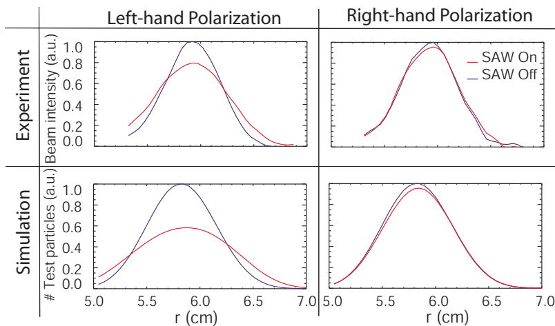
FIG. 6. (Color online) Comparison of fast-ion resonance effect with left-hand and right-hand polarizations.
