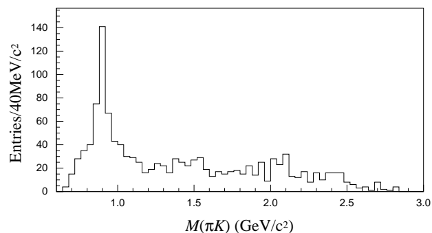
FIG. 4. The \pi^+K^- invariant mass distribution for \psi(2S) \rightarrow \pi^+\pi^-K^+K^- events (four entries/event).
