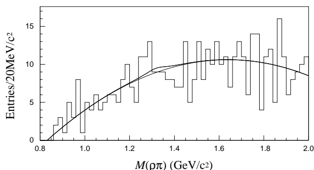
FIG. 3. The \rho\pi invariant mass distribution for events of the type \psi(2S) \rightarrow \rho^0\rho^\pm\pi^\pm . The curve shows a fit to quadratic background plus an a_2 resonance (see text).
