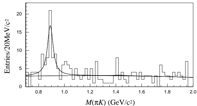
FIG. 5. The invariant mass distribution for \pi^+K^- tracks recoiling against a K^{*0} for \psi(2S) \rightarrow \pi^+\pi^-K^+K^- events. The curve shows a fit to quadratic background plus K^{*0} and K_2^{*0} resonances (see text).
