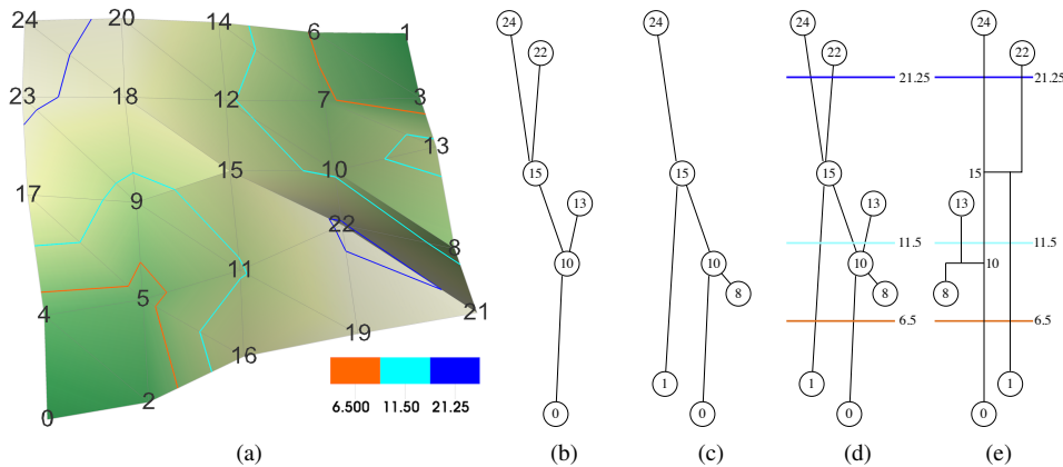
Figure 1: (a) Landscape and select isolines. (b), (c) Join and split tree record where maxima and minima respectively “meet.” (d) The branch decomposition is a hierarchical representation of the contour tree based on a simplification measure.
