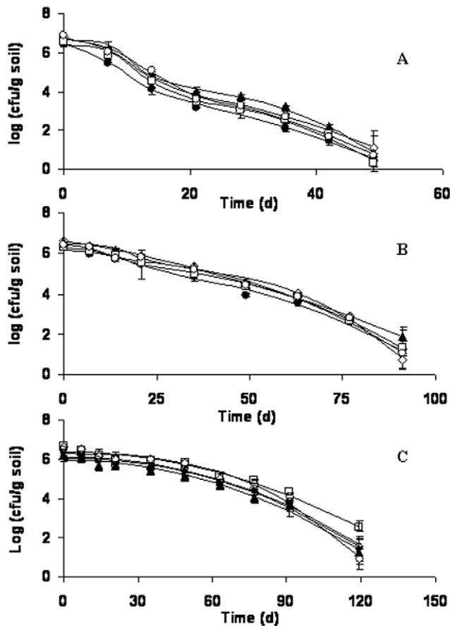
Figure 3. Survival of the wild type ( \bullet ) and its mutant derivatives, \Delta stx_1 ( \diamond ), \Delta eae ( \blacktriangle ), \Delta stx_2 ( \square ), and \Delta stx_1-2 ( \circ ), in loamy sand (3A), sandy loam (3B), and silty clay (3C). The data represent the average of triplicate experiments. doi:10.1371/journal.pone.0023191.g003
