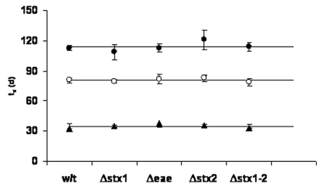
Figure 5. T_d values calculated from the double Weibull model for wild type and its mutants derivatives in loamy sand ( \blacktriangle ), sandy loam ( \circ ), and silty clay ( \bullet ). The data represent the average of triplicate modeling of the raw survival data. doi:10.1371/journal.pone.0023191.g005
