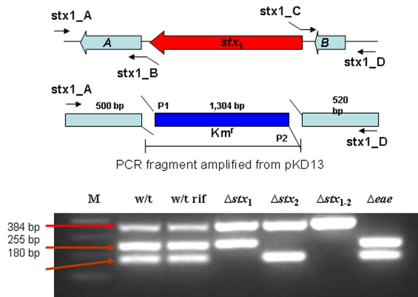
Figure 1. Construction of stx and eae mutants (top) and multiplex PCR confirmation of the mutant constructed (bottom). M represents 100 bp \lambda DNA ladder.
