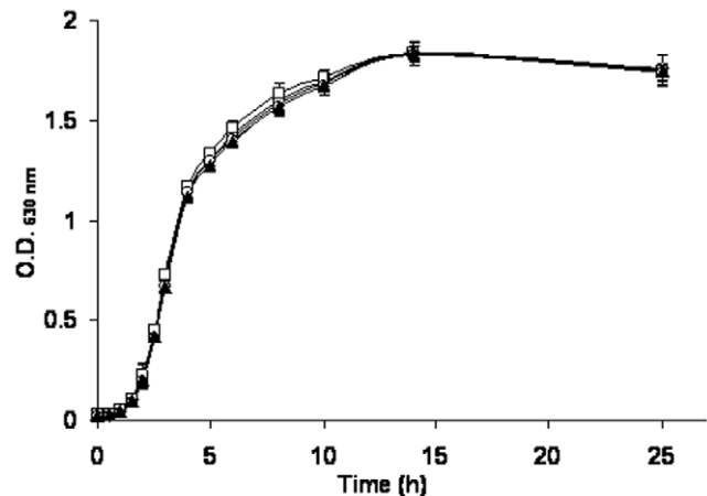
Figure 2. Growth curves of wild type strain (●) and its derivative mutants strains, \Delta stx_1 (◇), \Delta eae (▲), \Delta stx_2 (□), and \Delta stx_{1-2} (○). The data represent the average of triplicate measurements. doi:10.1371/journal.pone.0023191.g002
