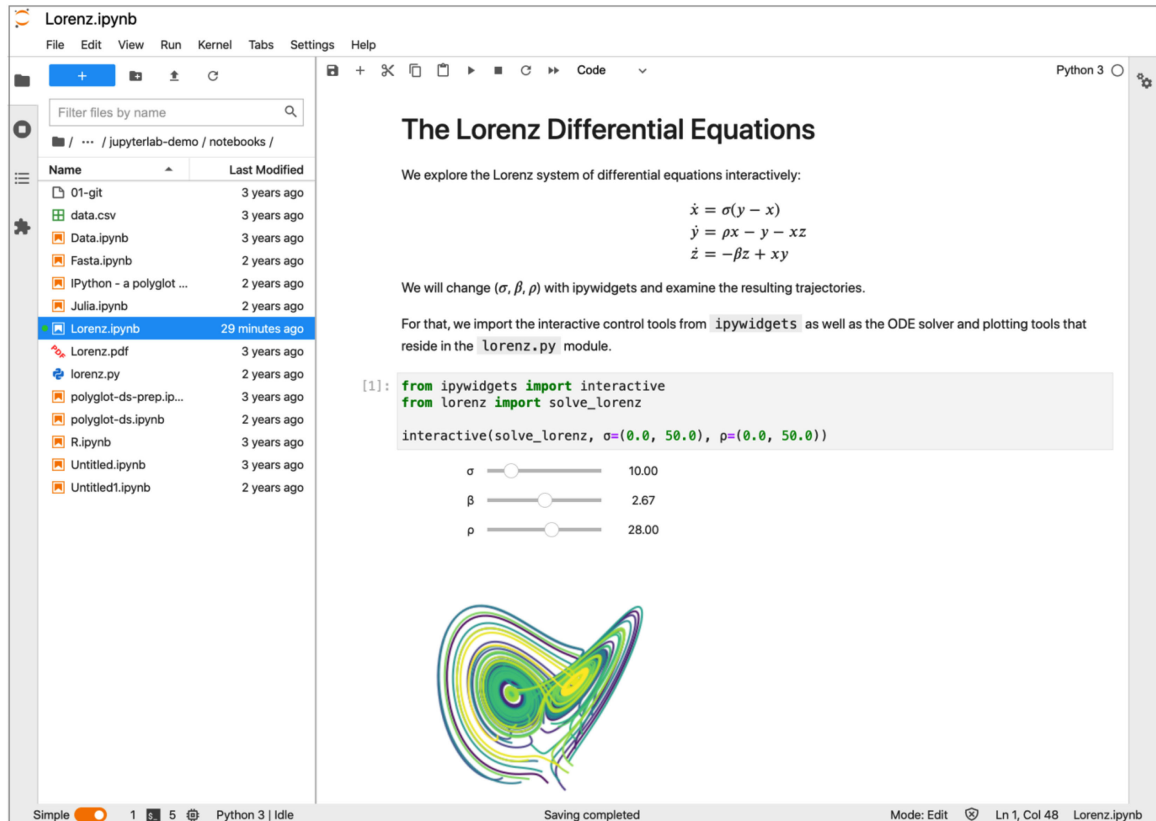
FIGURE 1. Example Jupyter notebook that solves the Lorenz differential equations, 7 open in JupyterLab. This notebook has live interactive code, headings, narrative text, equations, visualizations, and interactive controls that are organized into a human-centered computational narrative.
