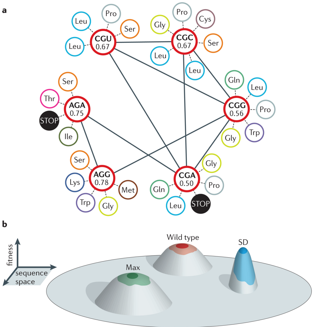
Figure 3. Using synonymous mutation to place populations in distinct fitness landscapes a A synonymous mutation alters the potential fitness impact of a subsequent mutation. Although two synonymous codons for arginine (such as AGG and CGG) are separated by a neutral A@C mutation, these codons differ in their propensity to mutate non-synonymously and non-conservatively. Shown are all six arginine codons (red circles) and, for each, the proportion of all potential mutations that would be non-synonymous. Synonymous mutations are indicated as solid lines, and non-synonymous mutations are indicated as dashed lines. b Large-scale synonymous mutation preserves the consensus amino acid sequence, but relocates viral populations in sequence space. When these viruses replicate
