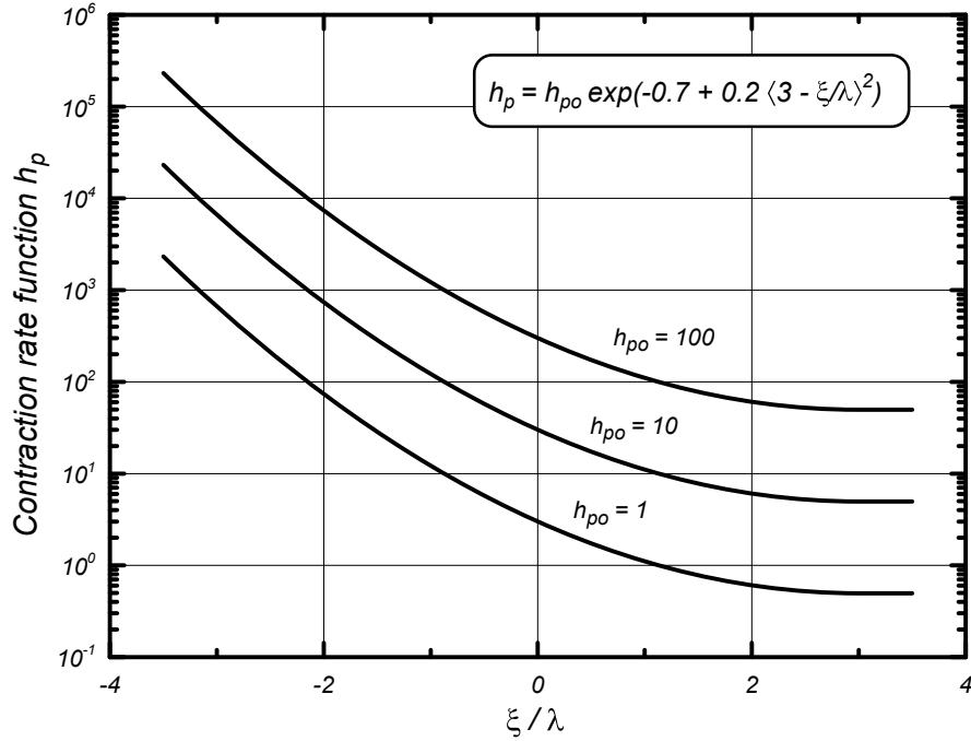
Figure 3. Variation of contraction rate function h_p with \xi/\lambda and contraction rate parameter h_{p0} .
