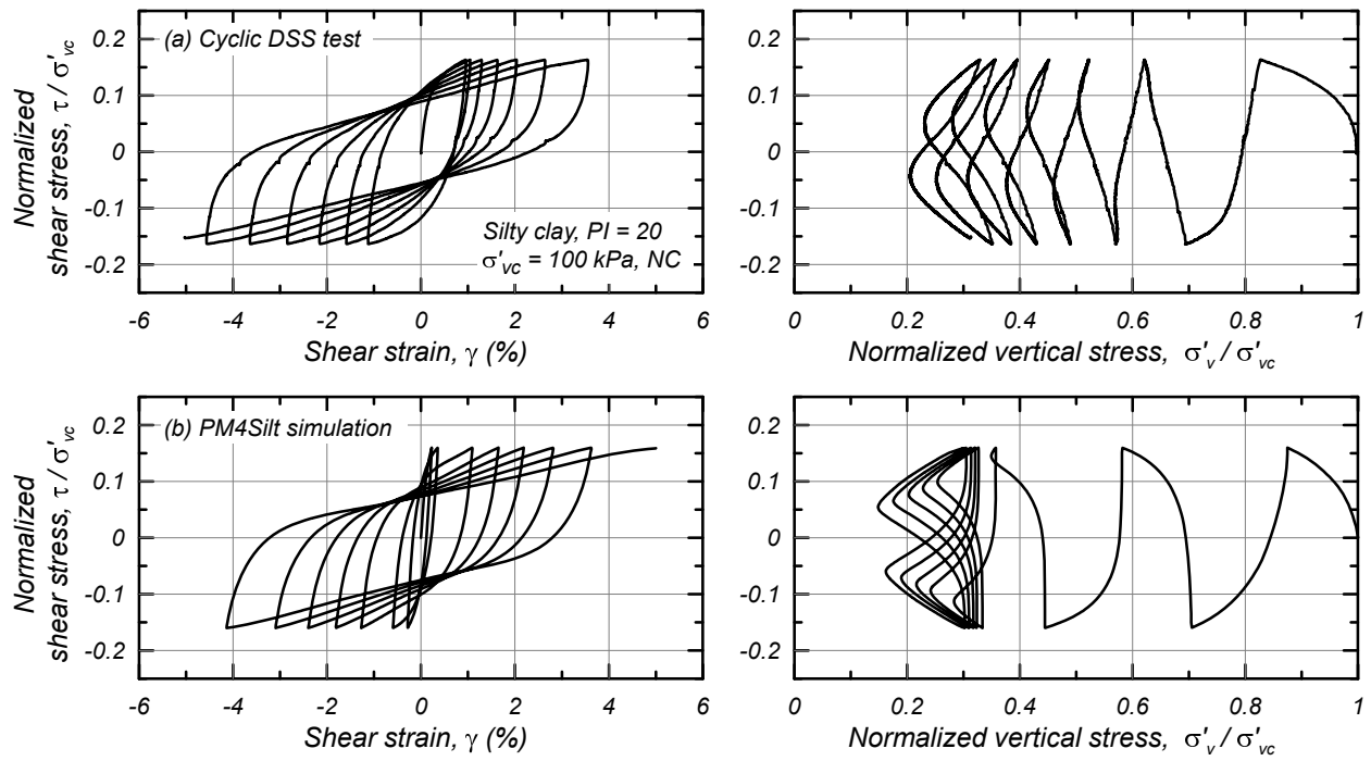
Figure 12. Stress-strain and stress path responses in cyclic undrained stress-controlled DSS loading for a slurry sedimented, normally consolidated silty clay with PI = 20 (Boulangier et al. 2018).
