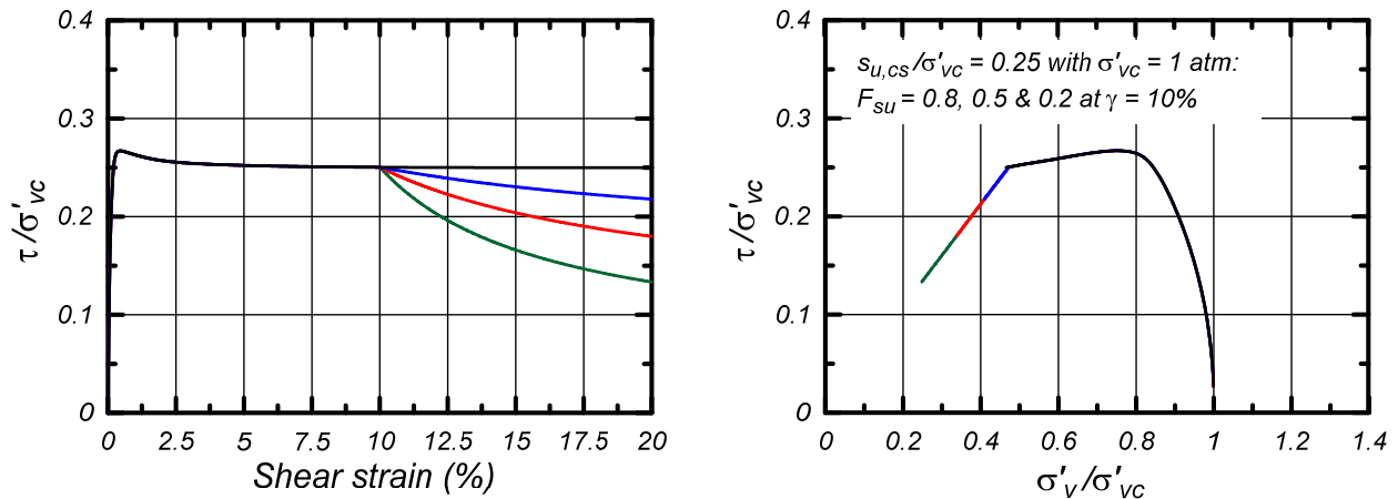
Figure 6. Effect of setting F_{su} = 0.8, 0.5, \text{ or } 0.2 at \gamma = 10\% on the response to further monotonic undrained DSS loading for a soil with s_{u,cs}/\sigma'_{vc} = 0.25 .
