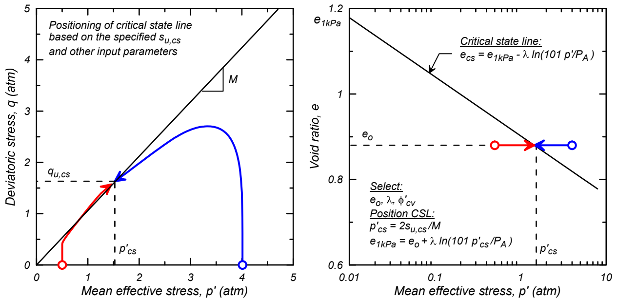
Figure 4. Procedure for positioning the critical state line based on the specified s_{u,cs} , along with simulated undrained responses for specimens with the same s_{u,cs} but starting at consolidation stresses corresponding to initially loose and dense of critical state conditions.
