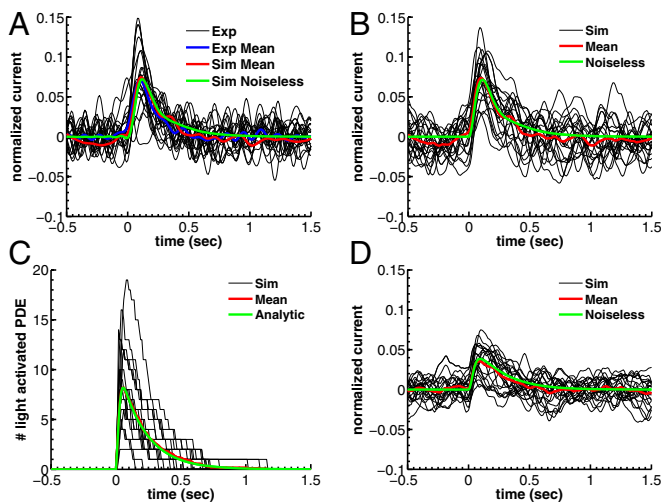
Fig. 4. Single-photon response for WT mouse rod. (A) Twenty suction-electrode recordings from a wild-type rod (black) with mean (blue). Currents are filtered at 20 Hz and normalized (dark current was 14.5 pA). Mean (red) and the noiseless simulation (green) from B are superimposed for comparison. SD of the dark current is 1.6%. Time, mean, SD, and CV of the peak current are 110 ms, 7.2%, 2.9%, and 2.9/7.2 \approx 0.40 . (B) Twenty single-photon response simulations (black) with mean (red) and noiseless simulation (green). Time, mean, SD, and CV of the peak current are 110 ms, 7.2%, 3.2%, and 3.2/7.2 \approx 0.44 . (C) Light-activated PDE (black) from B with mean (red) and with the analytic curve (green). Time, mean, and CV of the peak value are 55 ms, 8.2, and 0.49 (0.51 from SI Appendix, Eq. 58 ). (D) Twenty single-photon response simulations with increased calcium feedback. Parameters are as in A except B_{ca}=1 and r_{ca}=0 . SD of the dark current is 1.3%, in agreement with SI Appendix, Eq. 52 . Mean, SD, and CV of the peak current are 3.9%, 1.8%, and 1.8/3.9 \approx 0.46 .
