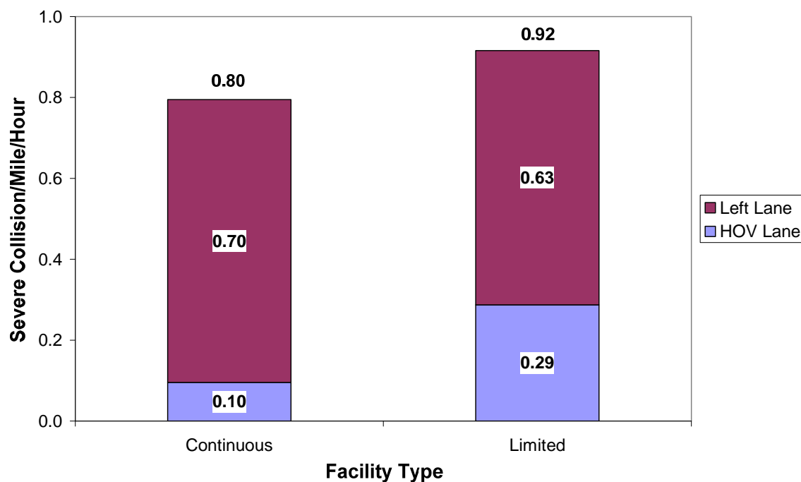
Attachment I A Comparison of Fatal and injury Collisions Per Mile Per Hour In HOV and Left Lanes (8 Study Routes)
