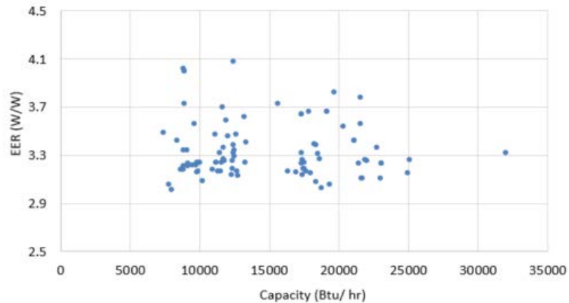
Figure 15. EERs for Common AC Cooling Capacities in Tunisia (no. of models = 99)
