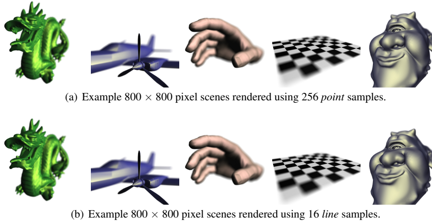
Fig. 11: 256 point samples (top) and 16 wagon-wheel line samples (bottom) per pixel produce nearly the same image, but line samples are about 4 times faster.
