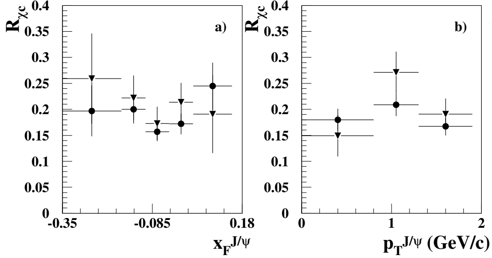
Figure 2.12: The \chi_c -to- J/\psi ratio measured by the HERA experiment as a function of x_F(J/\psi) (left) and p_T(J/\psi) (right). Triangles are from p + W , circles p + C . Figure from [81].
