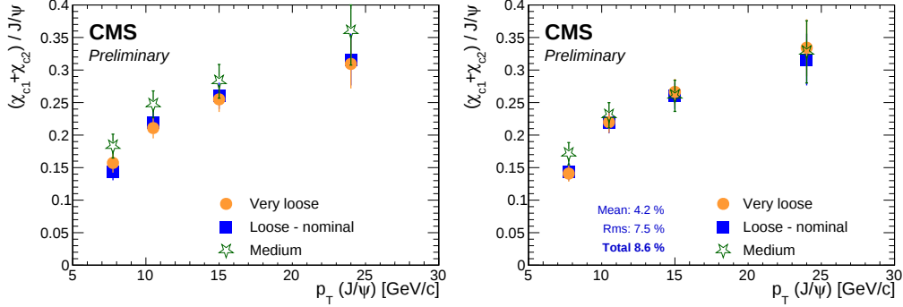
Figure 7.2: Left: The results as a function of p_T (J/\psi) for the various selections under the assumption that the peak shape stays the same. The results are not used since the assumption does not hold. Right: The same results with the full analysis procedure used.
