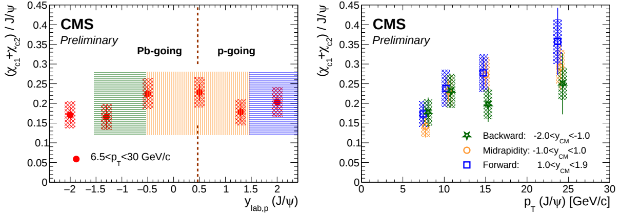
Figure 8.4: Left: \chi_c -to- J/\psi ratio plotted as a function of rapidity y_{\text{lab},p} (same data points as in Fig. 8.2). The shaded boxes show the rapidity ranges corresponding to those shown in the plot on the right, with the matching colors. Right: \chi_c -to- J/\psi ratio plotted as a function of p_T for three rapidity ranges defined in the center-of-mass frame: green: backward rapidity, Pb-going direction ( -2 < y_{\text{CM}}(J/\psi) < -1 ), orange: midrapidity ( -1 < y_{\text{CM}}(J/\psi) < 1 ), blue: forward rapidity, p-going direction ( 1 < y_{\text{CM}}(J/\psi) < 1.9 ).
