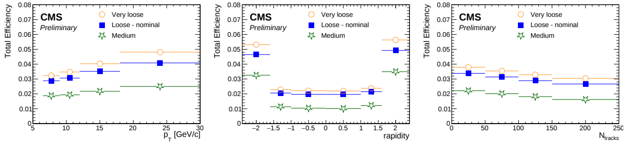
Figure 7.1: Efficiencies for the three conversion selections used in the study of the systematic uncertainty. Left, middle and right plot shows their dependence as a function of p_T , rapidity y_{\text{lab}} , and number of tracks, respectively.
