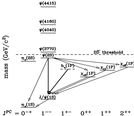
Figure 2.3: Charmonium family states. On the x -axis are their quantum numbers J^{PC} , and on the y -axis are their masses. Left: Full picture including recently discovered or speculative states. Right: Diagram showing only the main states. Figures from [24] and [25].
