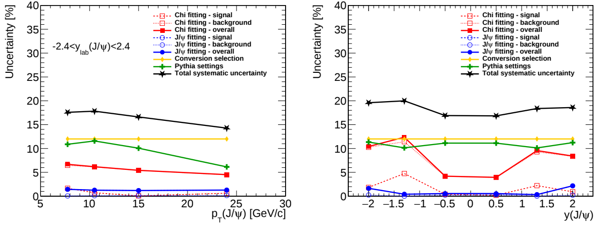
Figure 7.17: All systematic uncertainties plotted as a function of p_T(J/\psi) (left) and rapidity, y_{lab,p}(J/\psi) , (right).
