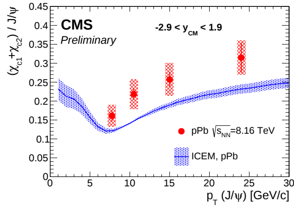
Figure 8.6: Comparison of the rapidity-integrated result (red points) to the calculation from the improved color evaporation model (blue line and band) in the same rapidity range [122].
