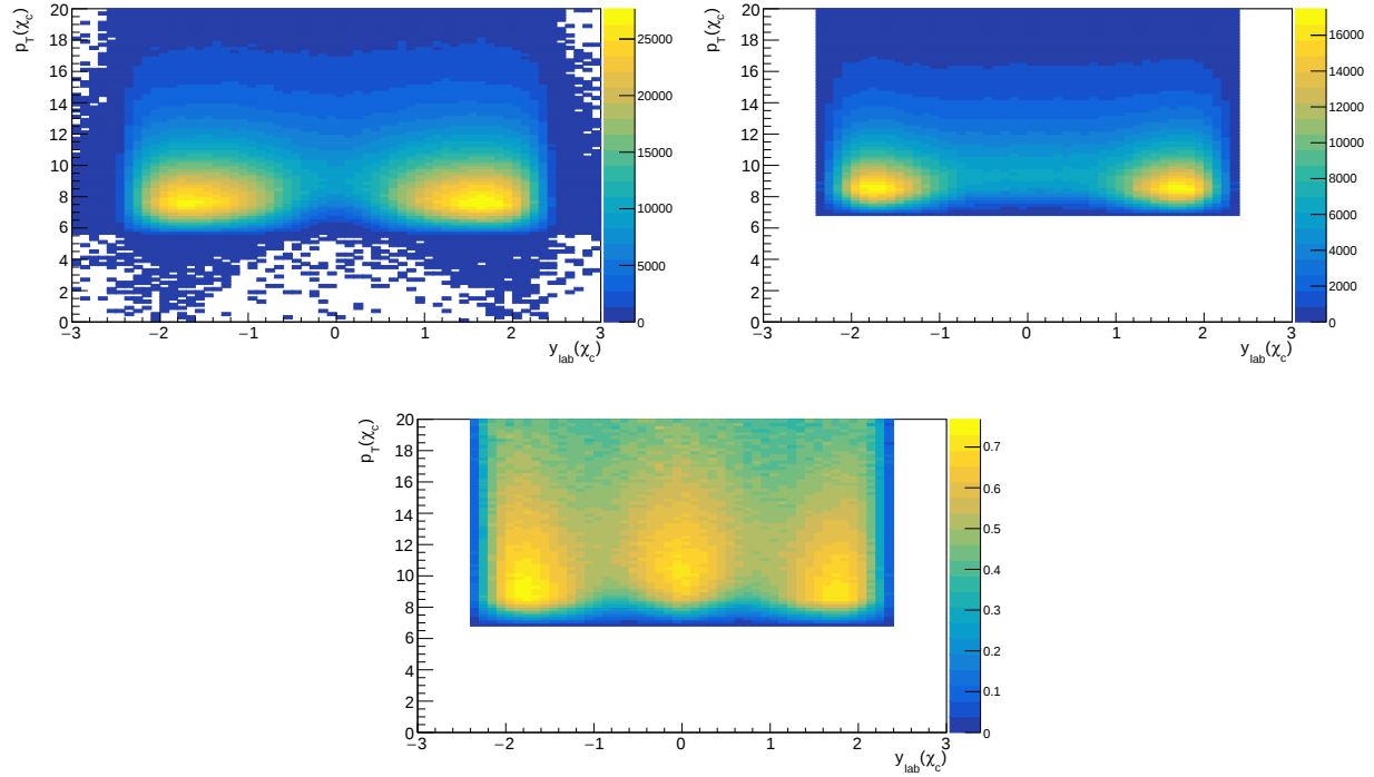
Figure 6.2: Acceptance plots for \chi_c , as a function of y_{\text{lab}} and p_T(\chi_c) . Top left: Distribution of generated \chi_c including pre-filter (see text for details). Top right: \chi_c passing acceptance cuts, which are acceptance cuts on daughter J/\psi , muons, and photon (no direct cut on \chi_c ). Bottom: Acceptance of \chi_c (specific to our MC).
