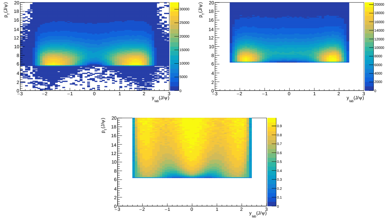
Figure 6.1: Acceptance plots for J/\psi , as a function of y_{\text{lab}} and p_T (J/\psi) . Top left: Distribution of generated J/\psi including pre-filter (see text for details). Top right: J/\psi passing acceptance cuts, including acceptance cuts on the daughter muons. Bottom: Acceptance of J/\psi (specific to our MC).
