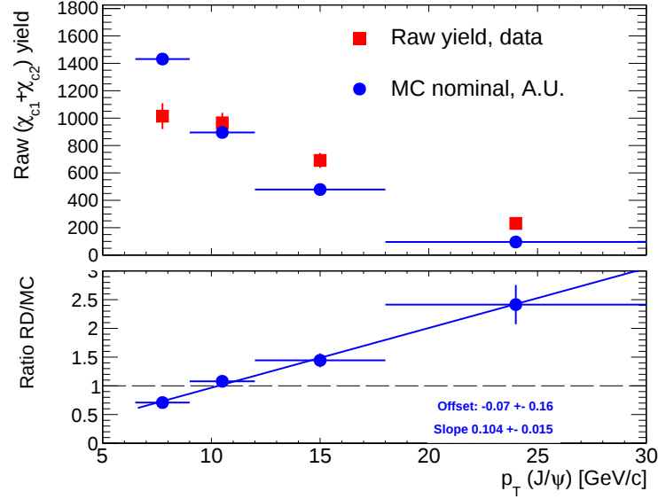
Figure 4.3: Top: The raw \chi_c yield as a function of p_T of the daughter J/\psi . The data points are in red, nominal MC in blue. The MC is scaled to match the integrated data counts. Bottom: Ratio of the data/MC, fitted with a linear function in blue.
