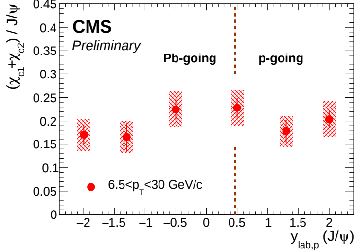
Figure 8.2: \chi_c -to- J/\psi ratio plotted as a function of rapidity y_{lab,p} . The rapidity is defined in the lab frame, with the p -going direction always being positive. The center of mass of the interacting system is shown by the brown dashed line.
