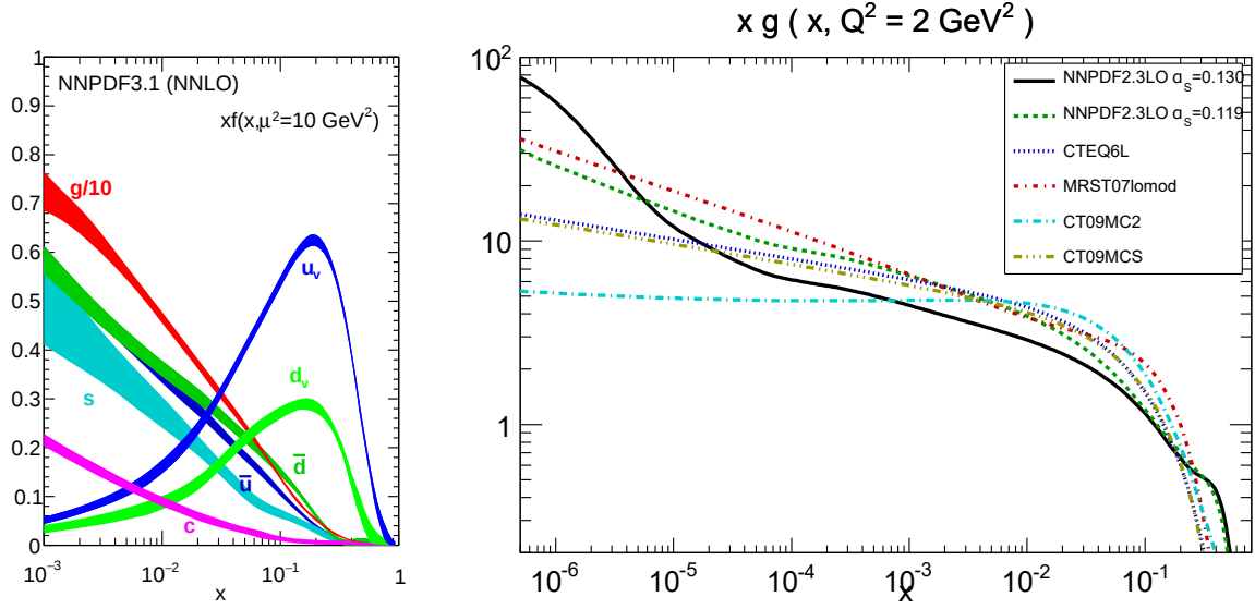
Figure 2.6: Left: Example PDFs for protons. The panel shows the updated NNPDF3.1. Figure from [60]. Right: Diagram showing various PDFs for gluons on a log-log scale. The most relevant PDF is the “NNPDF2.3LO, \alpha_s = 0.130 ”. It is the PDF that is used for the simulated samples for this analysis via the PYTHIA8 CUETP8M1 tune. Figure from [61].
