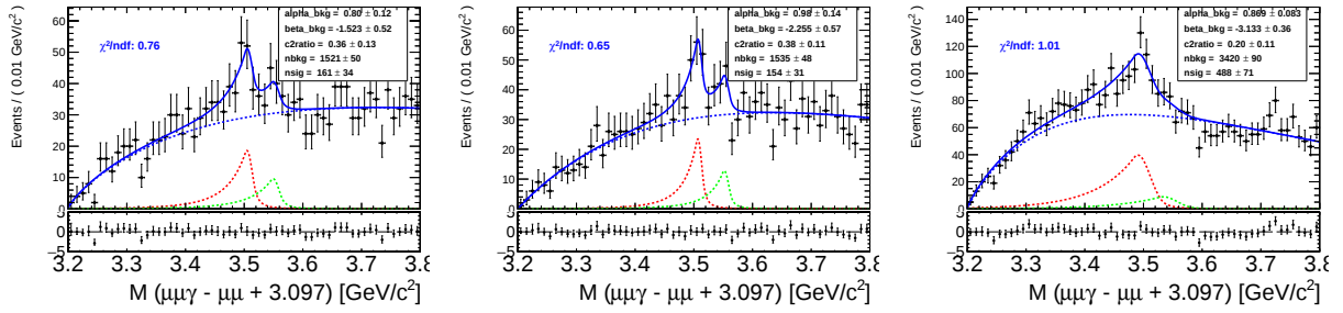
Figure 5.8: Examples of \chi_c fits for p_T binning for various subranges in y_{CM} . Lowest p_T bin ( 6.5 \text{ GeV} < p_T < 9 \text{ GeV} ) is shown in all three cases, as it has the most challenging background description. Left: Backward rapidity ( -2.0 < y_{CM} < -1.0 ). Middle: Midrapidity ( -1.0 < y_{CM} < 1.0 ). Right: Forward rapidity ( 1.0 < y_{CM} < 1.9 ).
