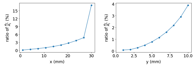
FIG. 7. Ratio of the two leading NAFF components increases with the initial particle amplitude in the horizontal (left) and vertical (right) planes for the DBA lattice.
