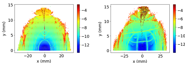
FIG. 5. DA of the DBA lattice with QI (left) and the NSLS-II lattice at nominal operation (right). The lattices have chromaticities of \xi = 7 and \xi = 2 , respectively. Colors indicate the tune diffusion obtained with the NAFF technique.
