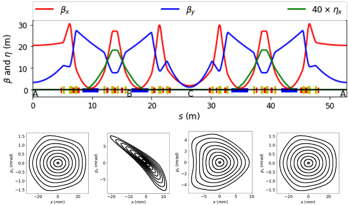
FIG. 16. Tori are near-circular only when observed at the long straight centers but could be distorted at other locations. The bottom four subplots are the tori observed at the locations “A-B-C-A,” respectively, as marked in the top subplot.
