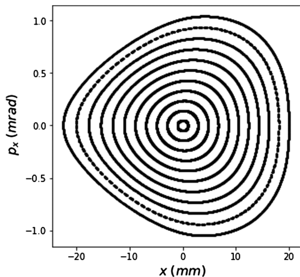
FIG. 20. Particle trajectories are confined to triangle-shaped tori, as confirmed by the tracking simulation. A nonsymmetric DA can be obtained with this technique.
