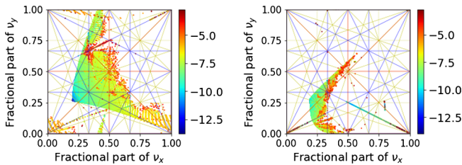
FIG. 9. Tune footprint of the NSLS-II DBA lattice with QI (left) and the nominal lattice for routine operation (right). The design working point is 33.22/16.26. Compared to the nominal lattice, a very large amplitude-dependent tune-spread is observed in the QI lattice, and various resonance lines can be crossed with narrow stop-band widths. Here colors indicate the tune diffusion, as in Fig. 5.
