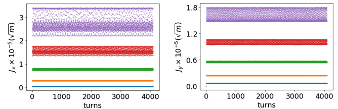
FIG. 6. Evolution of J_{x,y} in the DBA lattice starting from five different initial conditions in the horizontal (left) and vertical (right) planes.
