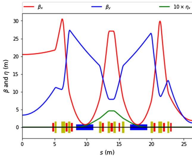
FIG. 4. Linear optics and magnet layout for one cell of the NSLS-II storage ring. The red blocks represent sextupoles. The strengths of six harmonic sextupoles were tuned during optimization of the nonlinear optics (Sec. II).
