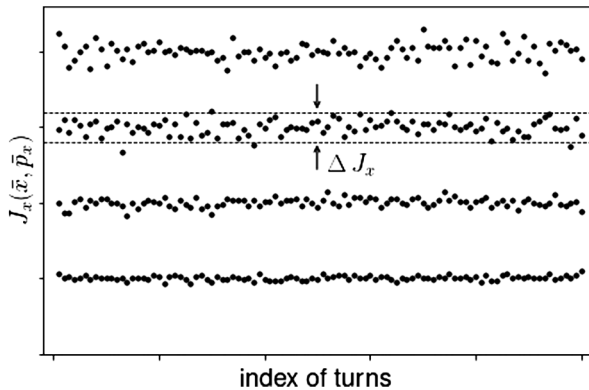
FIG. 2. Schematic illustration of the fluctuation of actions \Delta J_x starting from different initial amplitudes. Usually the fluctuations increase gradually with the initial amplitude.
