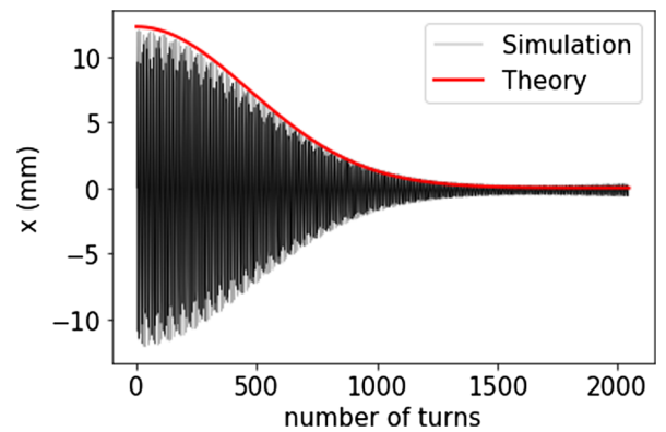
FIG. 17. After being kicked, the centroid of the beam will show a decaying oscillation. The red line is known as the decoherence factor in Eq. (6) and can be used to determine the local amplitude detuning coefficient \mu .
