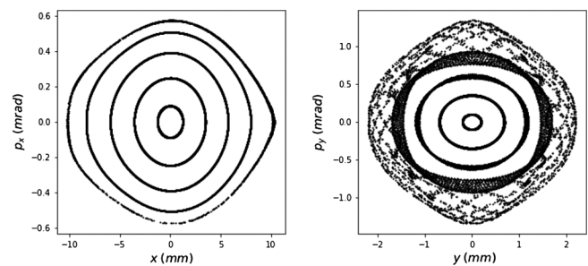
FIG. 14. Simulated trajectories of the MBA lattice in the horizontal (left) and vertical (right) phase space. The vertical trajectories begin to smear out from thin tori gradually, but some patterns are visible.
