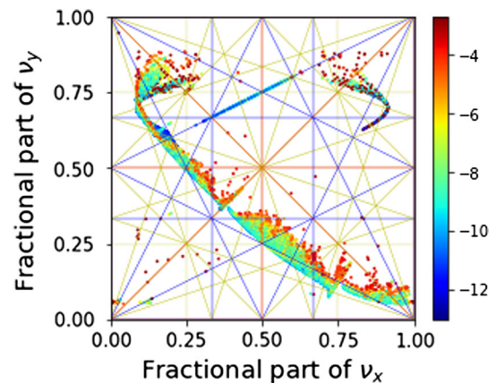
FIG. 15. Large amplitude-dependent tune spread is observed in the MBA lattice constructed with QI.
