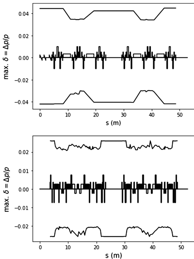
FIG. 18. Local momentum aperture of one supercell (including two mirror symmetric cells) for the constructed DBA (top) and MBA (bottom) lattices.
