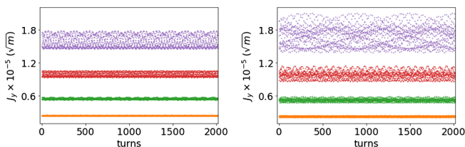
FIG. 10. Comparison of the vertical action fluctuations in the QI lattice (left) and the nominal NSLS-II lattice (right). Starting from the same initial conditions (x, p_x, y, p_y) , the action in the QI lattice has smaller fluctuations, despite the fact that the lattice has a high chromaticity \xi = 7 . The same feature can also be observed for the horizontal plane.
