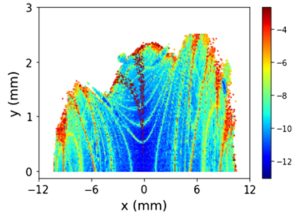
FIG. 13. DA of the MBA lattice in the transverse x - y plane colored with the tune diffusion.
