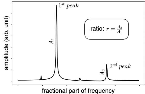
FIG. 3. Schematic illustration of the spectrum obtained from turn-by-turn trajectory data \bar{x} \pm i\bar{p}_x . The ratio between the amplitudes of the two leading frequencies \frac{A_2}{A_1} is the objective to be minimized to suppress the orbit tune diffusion.
