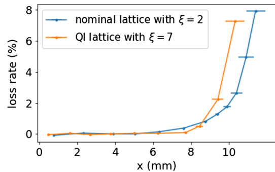
FIG. 11. Measured dynamic aperture of the DBA lattice with QI (yellow) and the NSLS-II lattice at nominal operation (blue). The lattice chromaticities are \xi = 7 and \xi = 2 , respectively.
