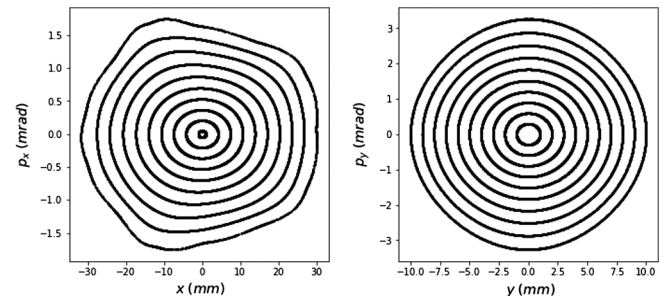
FIG. 8. Simulated trajectories of the DBA lattice starting from different initial conditions in the horizontal (left) and vertical (right) phase space. Within the DA, although the trajectories deviate from the Courant-Snyder ellipse, they are still confined to thin tori.
