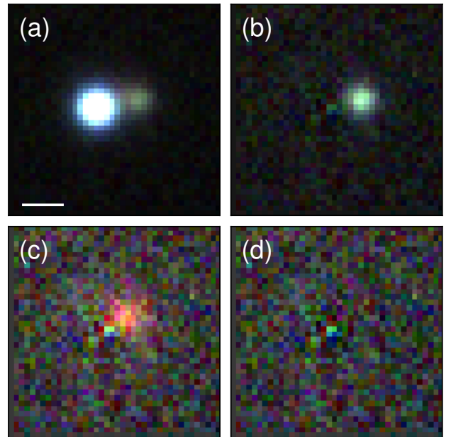
Figure 11. DES griz stacked model for DESJ2349-4518; (a) data, (b) subtraction of image A and lensing galaxy, (c) subtraction of both quasar images, and (d) subtraction of all components. The white scale bar is 2 arcseconds.
