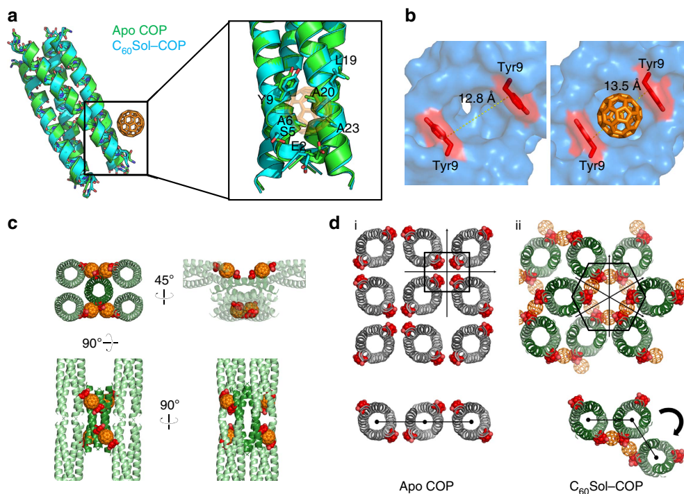
Figure 2 | COP crystal adjusts to incorporate fullerene. (a) Superposition of apo COP (green) and C 60 Sol-COP (cyan) shows no significant structural changes in the helix bundle. Side-chain differences around the fullerene-binding site are highlighted in the box. (b) The distance between aromatic Tyr9 residues adjusts in C 60 Sol-COP to incorporate the fullerene. (c) Different views of the COP-fullerene lattice. (d) Significant changes in the crystal lattice between COP alone and C 60 Sol-COP structures. Viewed from the top, C 60 Sol-COP forms a honeycomb structure (ii), whereas apo COP exhibits a tetrameric cube pattern (i).
