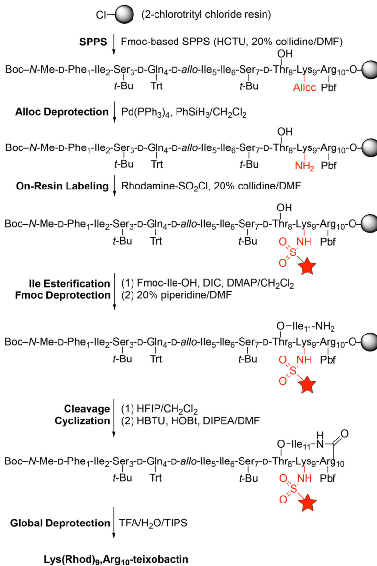
Scheme 1. Synthesis of Lys(Rhod) 9 ,Arg 10 -teixobactin
