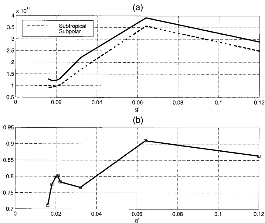
FIG. 11. (a) Area-weighted variance of the zonally averaged temperature variance as a function of the reduced gravity g' for the subtropical (dashed) and subpolar (solid) gyres. (b) Ratio of the subtropical to subpolar area-weighted variance of the zonally averaged temperature.
