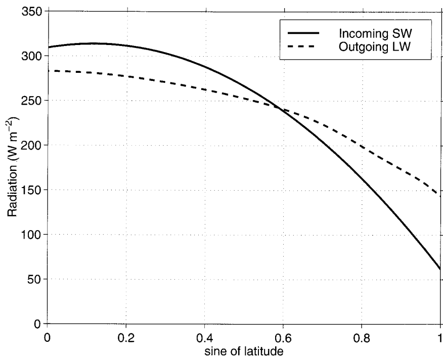
FIG. 1. Zonally averaged incoming shortwave radiation \langle Q_i \rangle and time- and zonally averaged outgoing longwave radiation \langle Q_o \rangle at the top of the atmosphere ( \text{W m}^{-2} ), as a function of the sine of the latitude for run 5.
