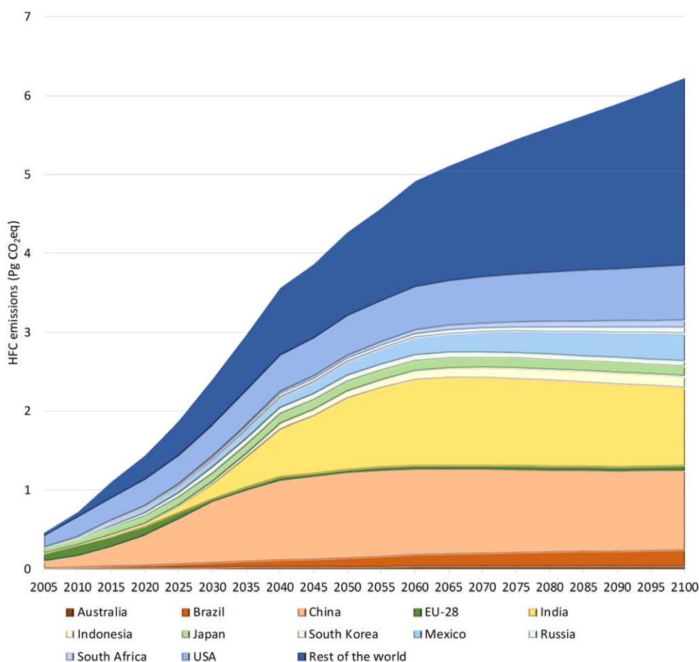
Figure 2. Pre-Kigali SSP3 baseline HFC emissions by regions.
