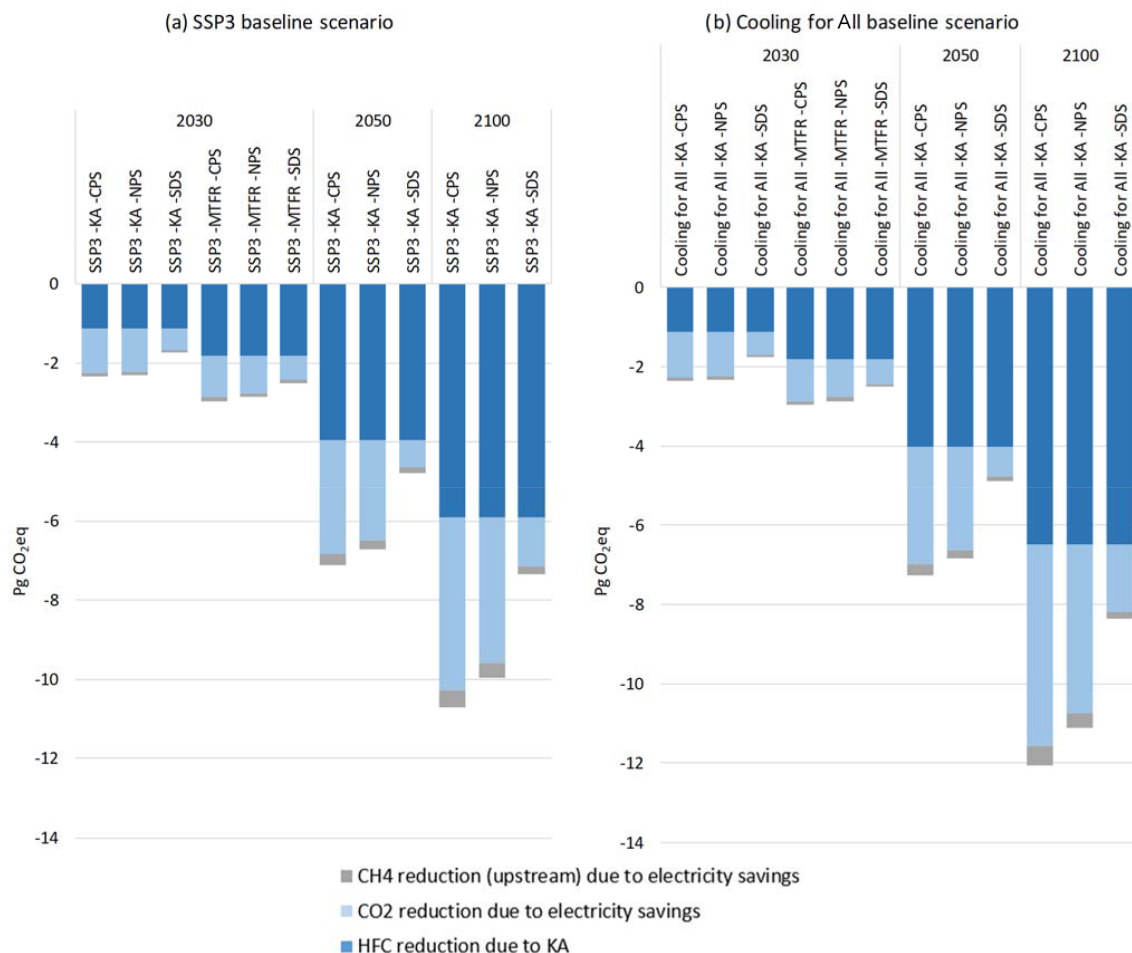
Figure 6. Greenhouse gas emission mitigation (in Pg CO 2 eq) due to enhanced energy efficiency benefits under Kigali amendment (KA) in the alternative scenarios with respect to the (a) SSP3 baseline scenario and (b) Cooling for All baseline scenario. In 2050 and 2100 differences between KA and maximum technically feasible reduction (MTRF) scenarios are negligible.
