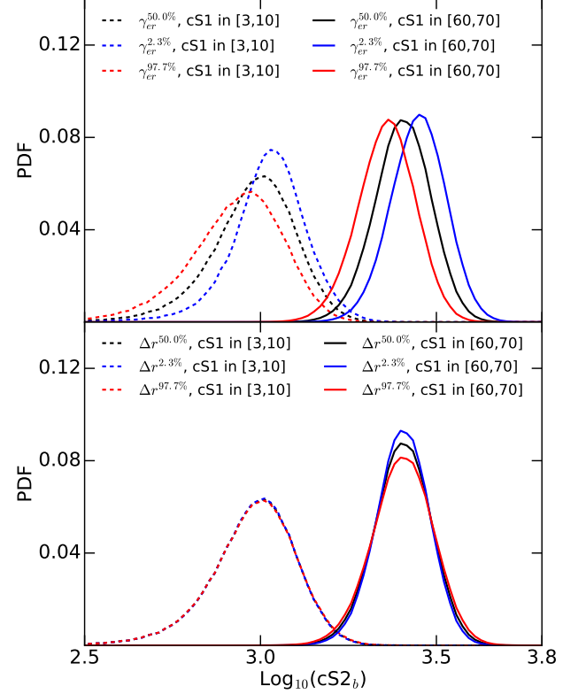
FIG. 4: Variations in \log_{10}(\text{cS2}_b) distributions as \gamma_{\text{er}} (top panel) and \Delta r (bottom panel) vary, from the 2.3% to 50.0%, and then to 97.7% percentile of the signal model posterior, in different \text{cS1} ranges.
