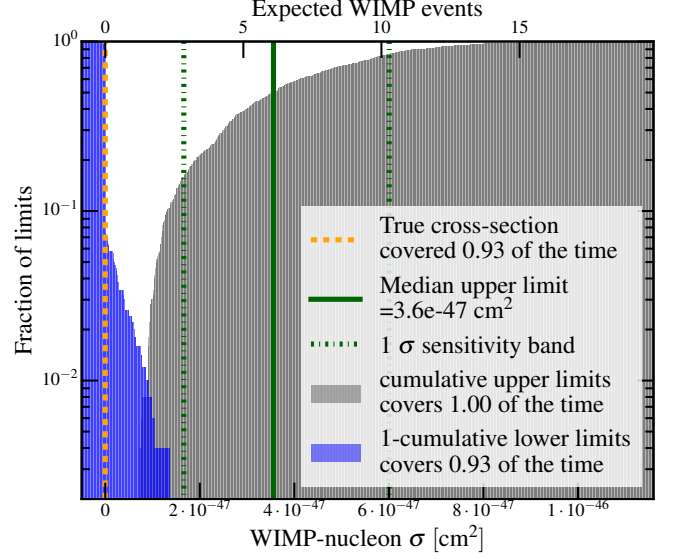
FIG. 9: Distribution of the lower (blue) and upper (gray) toy-MC limits on a 50 GeV/ c^2 WIMP cross-section. The upper (lower) limits are drawn as a cumulative (complementary cumulative) distribution, to show the fraction of limits that include a certain cross-section. The corresponding signal expectation value is shown on the upper horizontal axis. The toy-MC did not include a true signal, indicated with a dashed orange line at 0. All upper limits are above 0, and 0.93 of lower limits are equal to 0, giving a total estimated coverage of 0.93 for the 500 toy-MCs used in this example, part of the data-set used for figure 11. As the cross-section is constrained to be non-negative, the survival fraction below 0 is 1. Green solid and dot-dashed lines show the median upper limit and 1\sigma sensitivity band.
