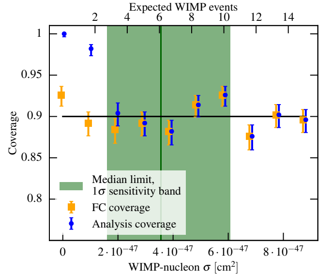
FIG. 11: Figure displaying the coverage of confidence intervals for the spin-independent 1 tonne-year analysis and a 50 \text{ GeV}/c^2 WIMP. Error-bars indicate 1\sigma confidence intervals around the best estimate. Orange squares show the result using the profile construction, while the blue circles show the coverage of the XENON1T analysis including the 3\sigma threshold for reporting upper limits. The upper and lower x-axes show the WIMP cross-section and expectation (setting \epsilon = 1 ) respectively, and the green band and line highlight the sensitivity and 1\sigma band of upper limits for the analysis.
