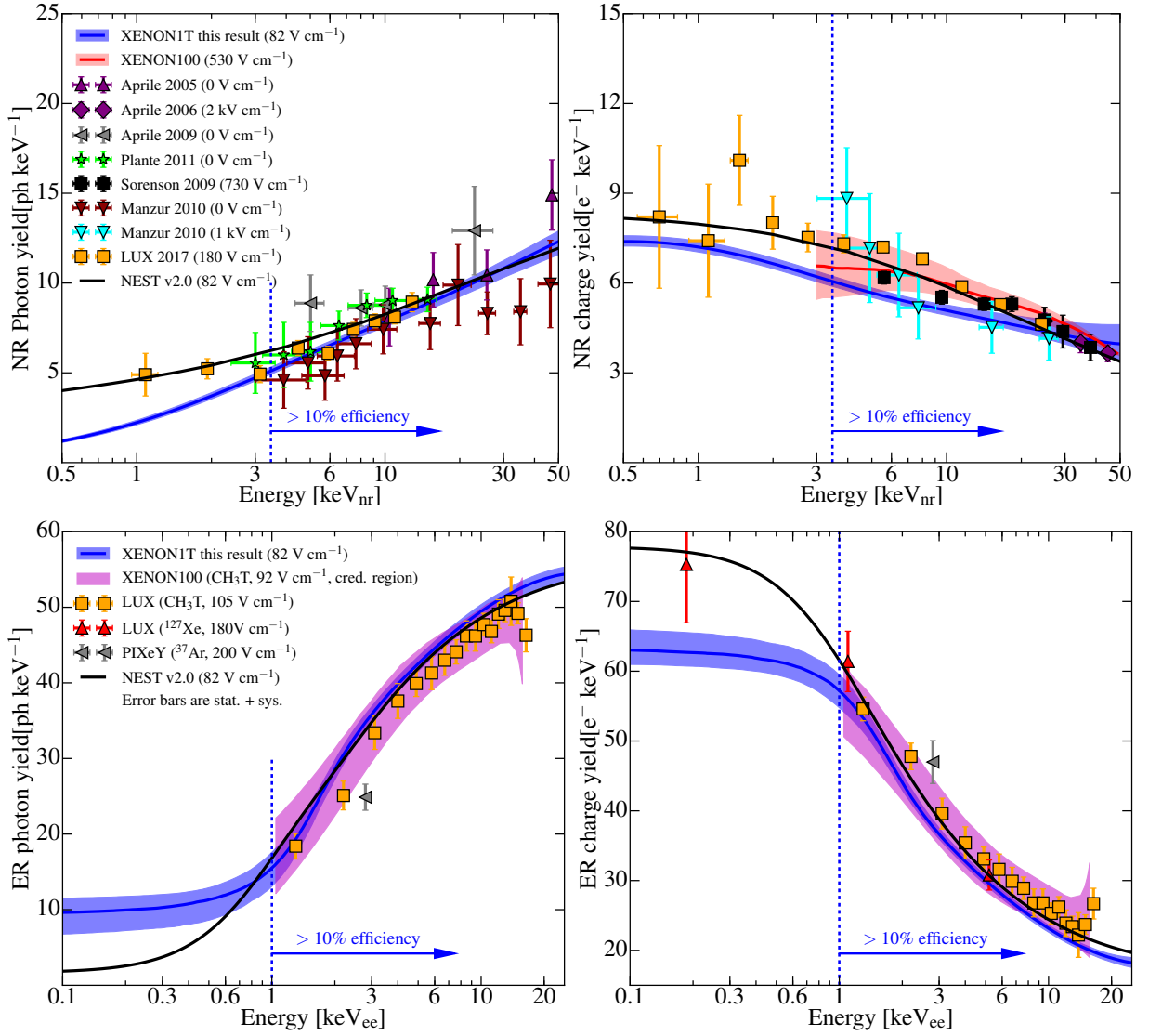
FIG. 1: Mean photon and charge yields of NR (upper panels) and ER (lower panels) in the XENON1T calibration data fit. The blue solid line and shaded region represent the point estimation and 15%-85% credible region, respectively, of the posterior. Data points for upper panels are from fixed-angle neutron scattering measurements [22–28]. Results of XENON100 [17] using data-Monte Carlo (MC) matching on the ^{241}\text{AmBe} calibration method are shown with the red solid line and shaded region. The best fit from NEST v2.0 [21] is shown with the black solid line. The measurements from [19, 20, 29, 30] are shown along with the best fit of NEST v2.0 [21] in lower panels. The vertical dashed blue lines indicates the energy threshold for XENON1T NR and ER calibrations, below which the detection efficiency drops to less than 10%.
