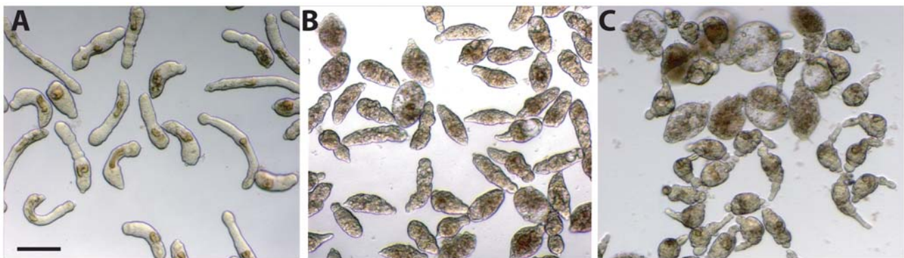
Figure 2. Examples of the different and multiple phenotypes manifest by schistosomula exposed to chemical insult. Worms were exposed for 7 days to 1 \mu M of either the schistosomicidal cysteine protease inhibitor, K777 (B), or the current chemotherapy, PZQ (C), and compared to controls with DMSO alone (A). Phenotypes ascribed are ‘dark/dead’ for K777 and ‘overactive/degenerated but mobile’ for PZQ. Images were captured using a Zeiss Axiovert 40 C inverted microscope (10 \times objective) and a Zeiss AxioCam MRC digital camera controlled by AxioVision 40 version 4.5.0.0 software. Scale bar = 0.2 mm. doi:10.1371/journal.pntd.0000478.g002
