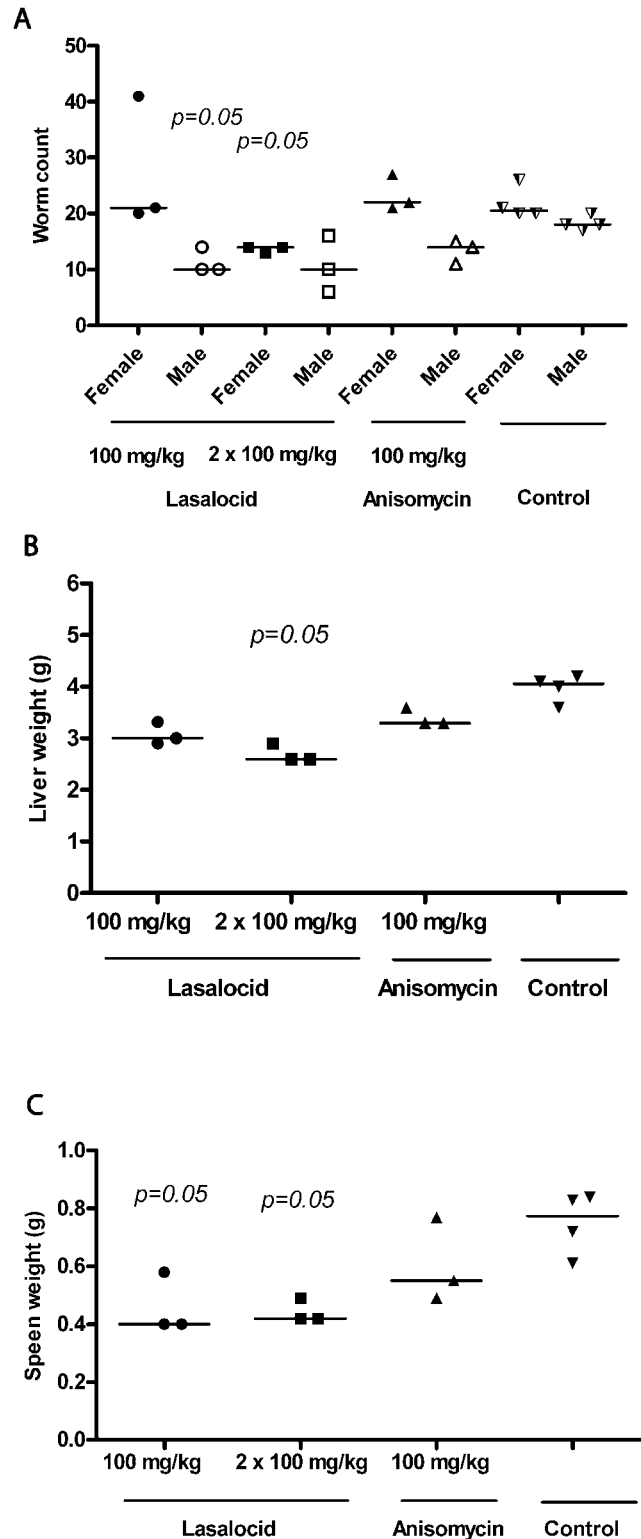
Figure 6. Effect of lasalocid sodium and anisomycin on male and female worm burdens, and organ pathology (as measured by weight) in mice infected with S. mansoni . Compounds were administered orally QD or BID at the doses indicated for 4 days 42 days after infection with 140 S. mansoni cercariae. Points represent data from individual treated or untreated (control) infected mice. The horizontal bars represent median values. Significance ( p ) values are indicated where p \leq 0.05 . Egg burdens were calculated as single values per treatment group (see text for details). doi:10.1371/journal.pntd.0000478.g006
