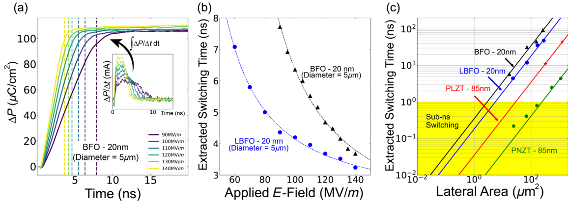
FIG. 2. Panel (a) shows the polarization transient, determined by integrating the difference between the switching and nonswitching current response in the system (inset). Dashed vertical lines show extracted switching time, defined as the time when polarization reached 90% of saturation. (b) shows experimentally observed switching times for 20 nm-thick BiFeO 3 (BFO) and 20-nm-thick Bi 0.85 La 0.15 FeO 3 (LBFO) as a function of applied field. The data reveals low-ns switching (dashed lines provide a guide to the eye). Panel (c) shows switching time as a function of area for the following samples: 20 nm BiFeO 3 (BFO), 20 nm Bi 0.85 La 0.15 FeO 3 (LBFO), 85 nm Pb 0.9 La 0.1 [Zr 0.2 Ti 0.8 ]O 3 (PLZT) and 85 nm Pb[Nb 0.04 Zr 0.29 Ti 0.67 ]O 3 (PNZT). Solid lines are linear best fits. The data shown are at an applied field of 95, 95, 26, and 60 MV/m for BFO, LBFO, PLZT, and PNZT, respectively. We include similar data for all samples and applied fields in this study (Supplemental Material [19], Fig. S4).
