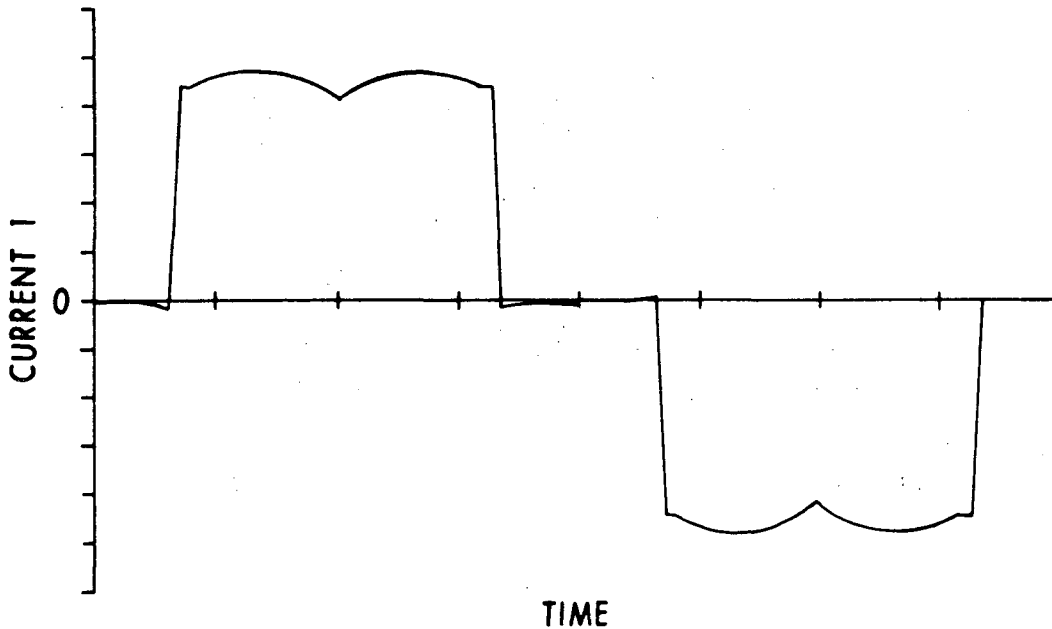
Item (c) - Computer Simulated Three-Phase Full-Wave Bridge Current Input
