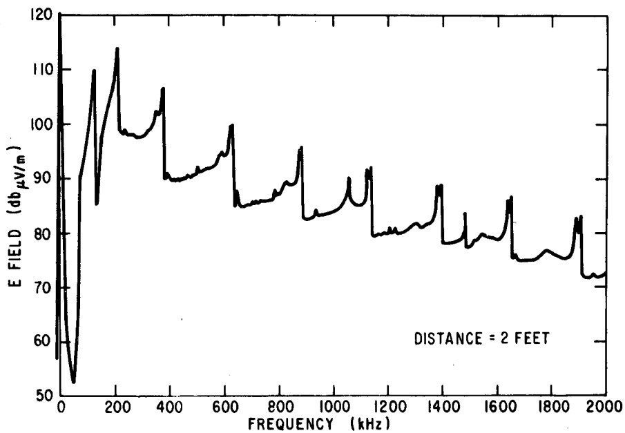
Figure #3 Radiated electric field intensity from typical unmodified Soleniodal Electric Field lamp.
