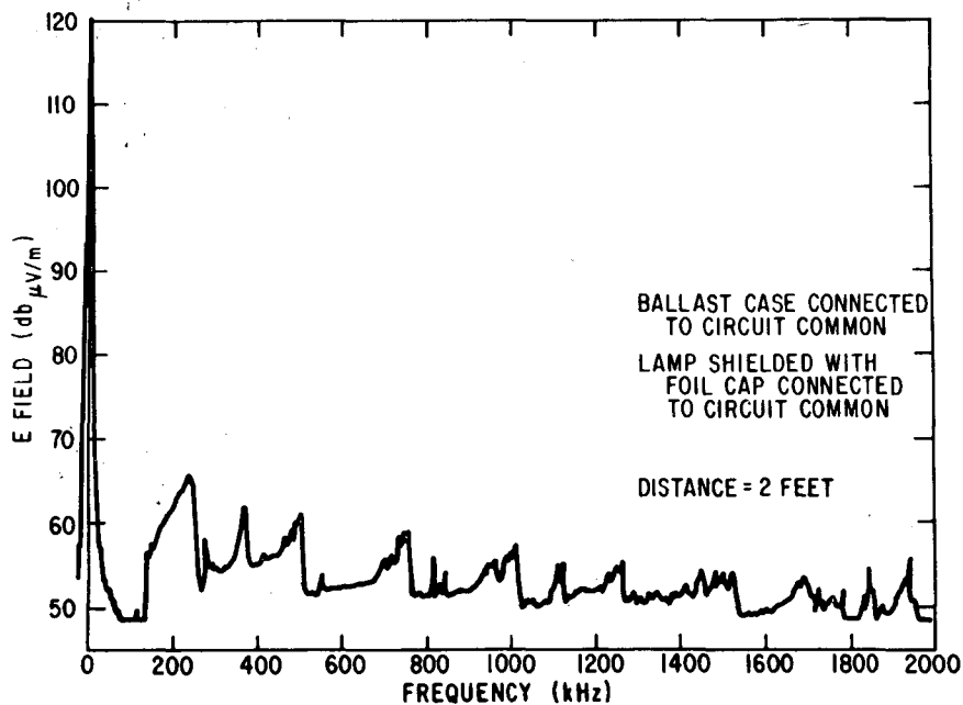
Figure #7 Radiated electric field from Solenoidal Electric Field lamp with ballast case and foil lamp shield connected to circuit common.
