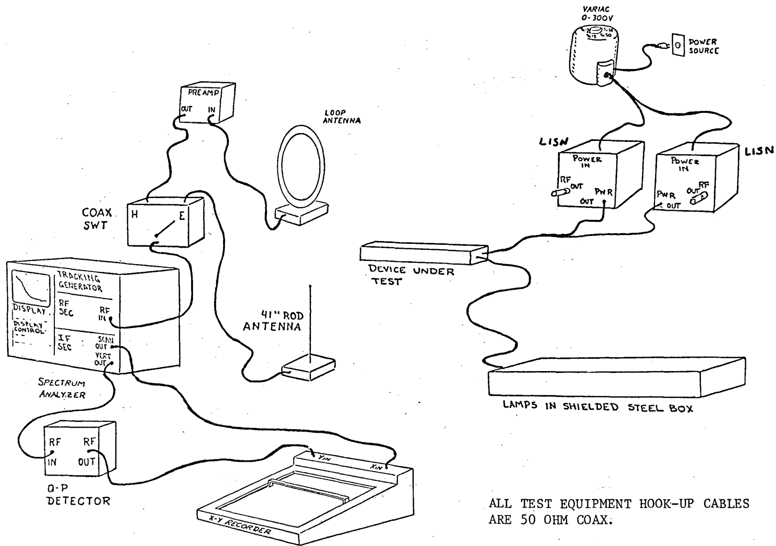
RADIATED EMI TEST PROTOCOL. FIG. 2
