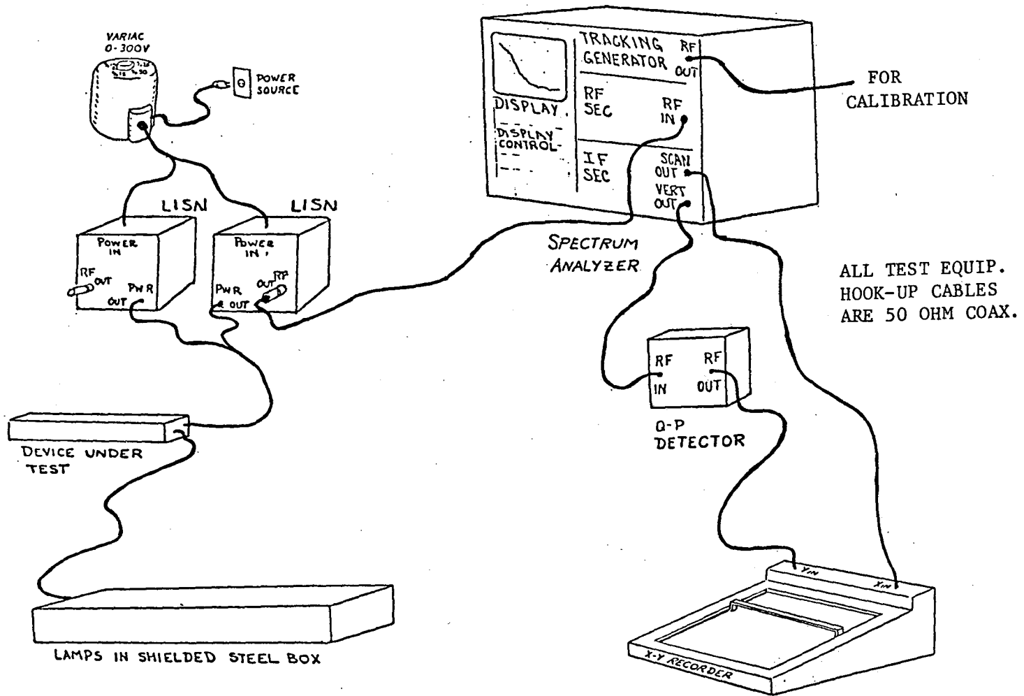
CONDUCTED EMI TEST PROTOCOL FIG.1.
