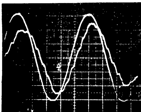
INPUT VOLTAGE AND CURRENT PHOTOGRAPHS OF A SHIPBOARD SEARCH RADAR SUPPLIED BY A 200 KW, 450 VOLT 400 HZ GENERATOR
