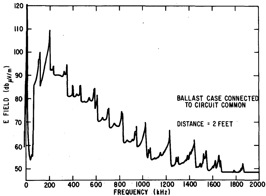
Figure #6 Radiated electric field from Solenoidal Electric Field lamp with ballast case connected to circuit common.
