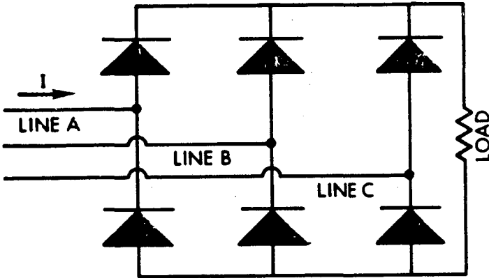
Item (c) - Computer Simulated Three-Phase Full-Wave Bridge Current Input
