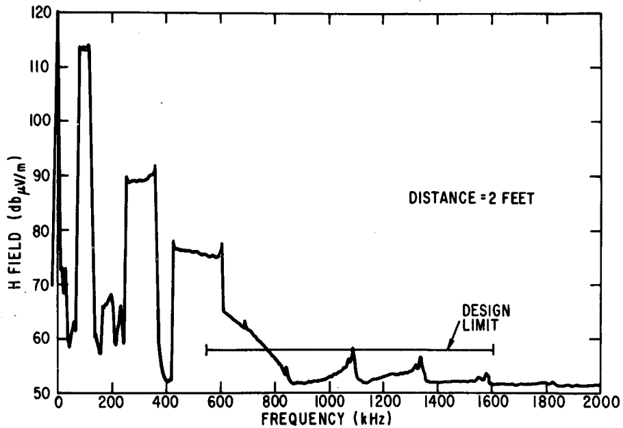
Figure #2 Radiated magnetic field intensity from typical Soleniodal Electric Field lamp (H field shown in equivalent E field units for far field radiation).
