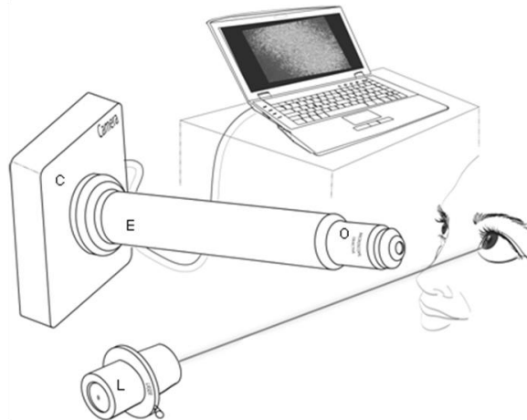
Fig. 1. The schematic of the FASIC setup is shown here. A 635nm low power (<1mw) laser is illuminated onto the cornea in order to measure the pre-corneal tear film thickness. The reflecting and scattering light is captured by a CMOS camera that is positioned in an angle with respect to the incoming light. A stack of 256X256 pixel images are streamed to a computer through a firewire cable for further analysis.
