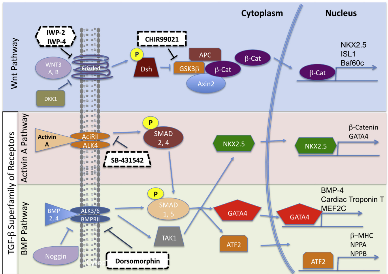
Fig. 1. A simplified schemata of the Wnt and TGF-β signaling pathways, which include molecular components that are targets to induce cardiac differentiation of PSC. Dashed boxes highlight small molecules that are currently used to efficiently drive cardiac differentiation of PSC.
