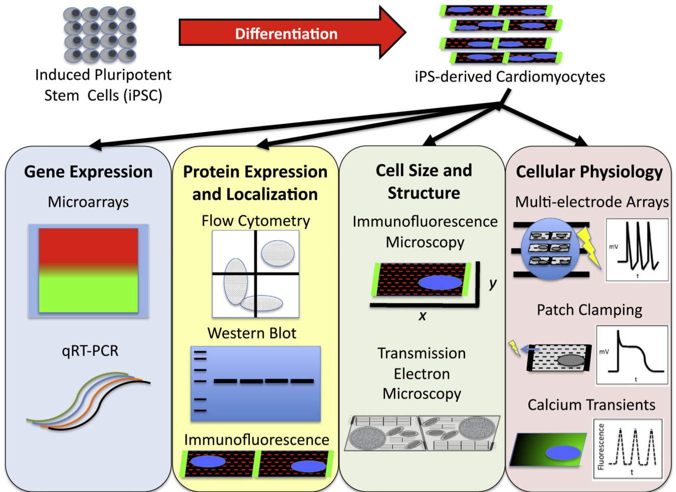
Fig. 2. Schemata of molecular, cellular, and functional techniques used for analysis of disease phenotypes in hiPSC-derived cardiomyocytes.
