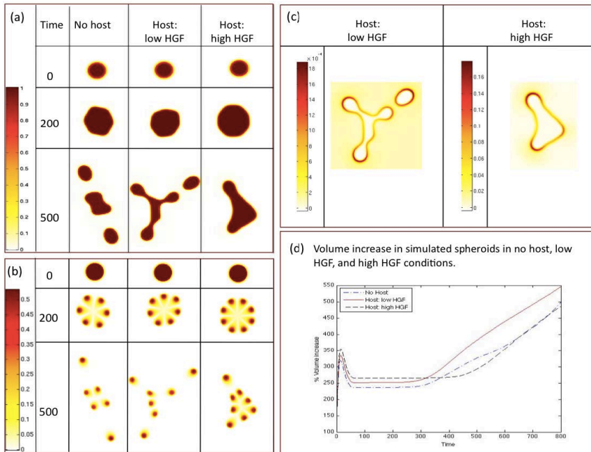
Fig. 3 Simulation results of tumor-host model: Visualization of numerical results of the mathematical formulation for incorporation of host factors (HGF) at low and high levels into a multispecies model for a total tumor, b stem cell fraction, and c HGF concentration (note difference in scale). d Tumor volume is increased in low HGF environment, but decreases in increased concentration of HGF
