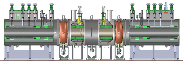
Figure 1: MICE beamline layout.
