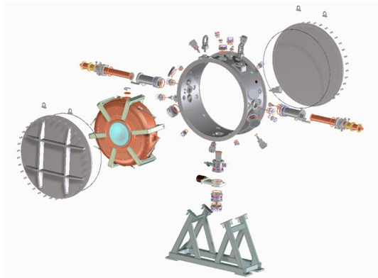
Figure 2: RF module exploded view.
