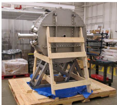
Figure 7: Vacuum vessels arrived at LBNL.
