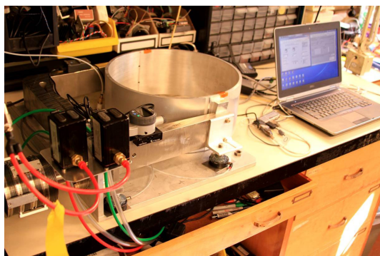
Figure 10: Actuator lifetime test.
