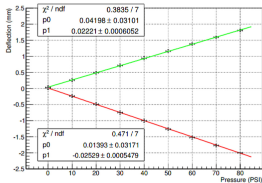
Figure 9: Actuator functional test: Deflection vs Applied pressure.
