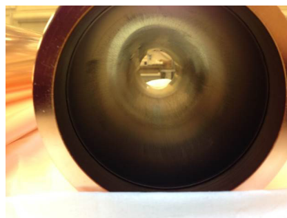
Figure 3: TiN coating of the inner surface of coax waveguide.
