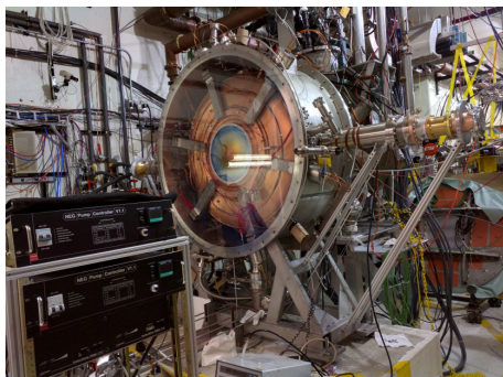
Figure 6: High power test of Single Cavity Module at MTA.
