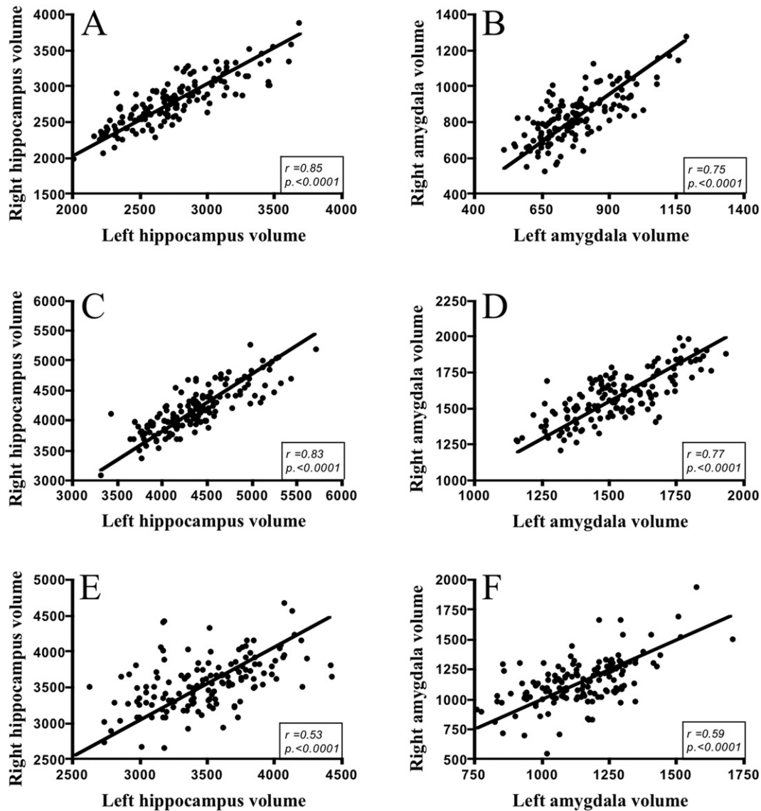
Fig. 7. Within-method correlations of left versus right structure volumes. A – Correlation between left and right hippocampus volumes segmented manually. B – Correlation between left and right amygdala volumes segmented manually. C – Correlation between left and right hippocampus volumes segmented automatically with FreeSurfer. D – Correlation between left and right amygdala volumes segmented automatically with FreeSurfer. E – Correlation between left and right hippocampus volumes segmented automatically with FSL-FIRST. F – Correlation between left and right amygdala volumes segmented automatically with FSL-FIRST. r – Pearson correlation coefficient.
