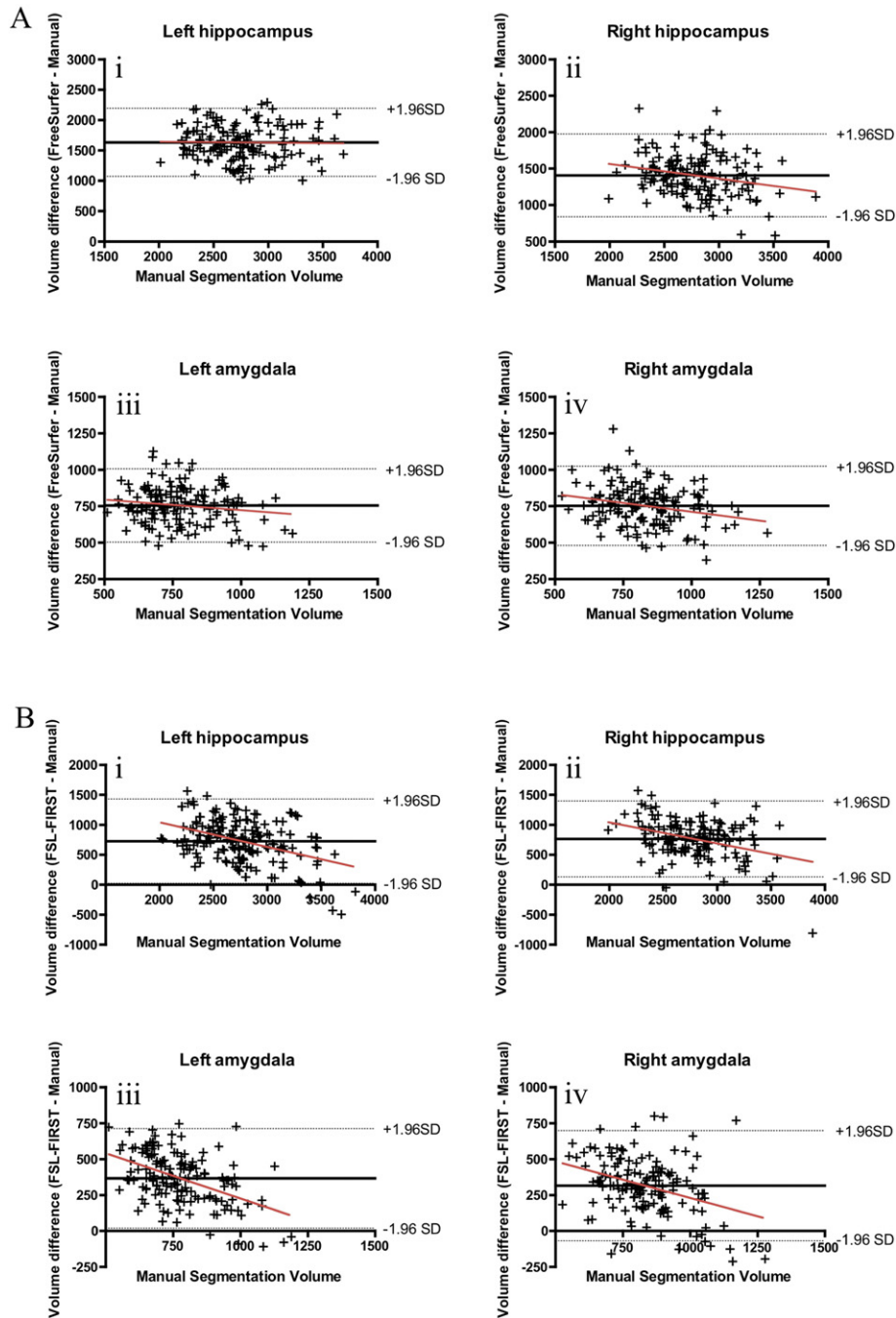
Fig. 8. Bland–Altman plots of volume difference estimation between manual segmentation and (A) FreeSurfer or (B) FSL-FIRST. Plots are presented separately for i – left hippocampus ii – right hippocampus, iii – left amygdala, iv – right amygdala. A red regression line was integrated to each plot to illustrate potential biases in volume estimation.
