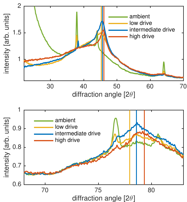
FIG. 4. Azimuthally integrated lineouts of the X-ray diffraction images shown in Fig. 3. Top: X-ray diffraction angles 2\theta = 22^\circ - 70^\circ . Bottom: X-ray diffraction angles 2\theta = 68^\circ - 83^\circ . The positions of the (111) and (220) diffraction peaks corresponding to the average diamond densities observed for the different drives [“low drive”: (4.05 \pm 0.07) g/cm 3 , “intermediate drive”: (4.14 \pm 0.06) g/cm 3 , and “high drive” (4.23 \pm 0.05) g/cm 3 ], which were inferred from the more accurate positions of the (111) reflection, are marked by vertical lines [(111) in top diagram, (220) in bottom diagram].
