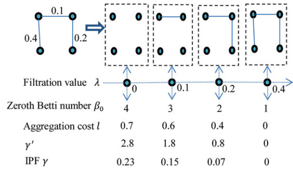
FIGURE 2 A computation example of topological features based on Figure 1. The top left is an MST T of weighted graph in Figure 1 left, followed by four nested trees \mathcal{B}(T,0) \subset \mathcal{B}(T,0.1) \subset \mathcal{B}(T,0.2) \subset \mathcal{B}(T,0.4) at four increasing filtration values 0, 0.1, 0.2, and 0.4, respectively. The topological features of the binary network, such as the zeroth Betti number and IPF, are varied according to the increase of filtration value \lambda [Color figure can be viewed at wileyonlinelibrary.com]
