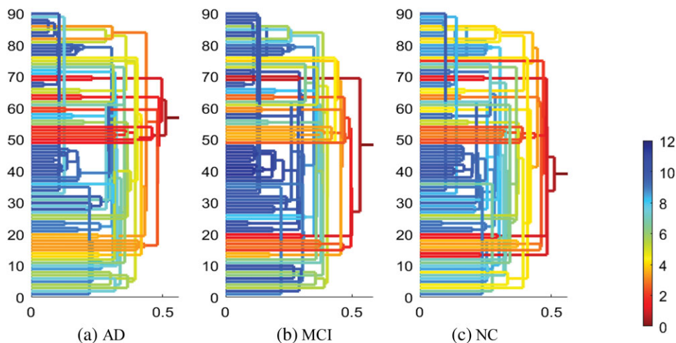
FIGURE 7 The single linkage dendrograms (SLDs) for 3 group means of (a) AD, (b) MCI, and (c) NC. The vertical and horizontal axes represent the node index and filtration value, respectively. The color of lines represents the total edge weight from current connected component to the giant component. The total weight from the giant component is 0. When individual components evolves to a fully connected component, the total edge weight decrease [Color figure can be viewed at wileyonlinelibrary.com]
