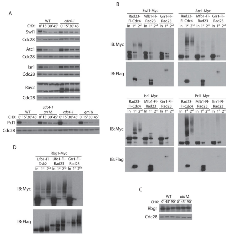
Figure 5. Ubiquitination of Cdc4 and Ufo1 candidate substrates (A) Myc-tagged Cdc4 candidate substrates were expressed in CDC4 cells or cdc4-1 temperature sensitive mutants. Cultures were simultaneously shifted from 23°C to 37°C and treated with CHX for the indicated number of minutes. Western blots were probed with anti-Myc (substrates) or anti-Cdc28 (loading control). A cdc4-1 grr1 double mutant was examined for Pcl1. (B) Western blots of two-step purifications performed on cell extracts expressing Rad23-FL-Cdc4 and Myc-tagged Swi1, Atc1, Isr1 or Pcl1, as in Figure 1. (C) The Ufo1 candidate substrate Rbg1 was Myc-tagged in UFO1 and ufo1 cells, treated with CHX for the indicated times, and examined by Western blot. (D) Western blot of two-step purifications performed on cell extracts expressing Ufo1-FL-Rad23, Ufo1-FL-Dsk2 or Grr1-FL-Rad23 together with Myc-tagged Rbg1.
