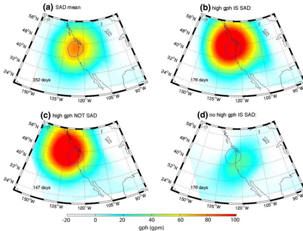
Fig. 5 a Mean 700 hPa geopotential height anomaly for days with the Santa Ana index greater than 5 \text{ m s}^{-1} . High geopotential height days are defined as days where the spatial average height anomaly in the region within the thin blue line is above 70 m. b Mean 700 hPa geopotential height anomaly for days with a high geopotential height anomaly and with SA greater than 5 \text{ m s}^{-1} . c Same as (b), but for days with SA less than 5 \text{ m s}^{-1} . d Mean 700 hPa geopotential height anomaly for days with SA greater than 5 \text{ m s}^{-1} but without a high geopotential height anomaly. The approximate geostrophic wind speed associated with the composite anomaly over Southern California is (a) 6 \text{ m s}^{-1} , (b) 8 \text{ m s}^{-1} (c) 6 \text{ m s}^{-1} and (d) 4 \text{ m s}^{-1}
