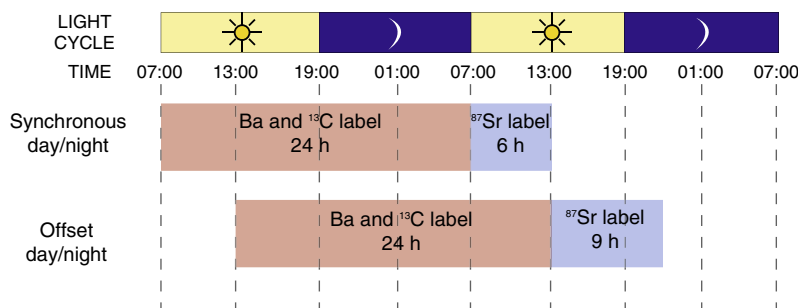
Fig. 2. Schematic diagram of two sets of labeling experiments: [Top] For O. universa specimens with 13 C label synchronous with day/night cycle, individuals calcified in Ba- and 13 C-labeled seawater for 24 h (07:00 to 07:00), then were transferred to 87 Sr-labeled seawater for 6 h of calcification. [Bottom] For O. universa specimens with 13 C label offset from day/night cycle, individuals calcified in Ba- and 13 C-labeled seawater for 24 h (13:00 to 13:00), then transferred to 87 Sr-labeled seawater for 9 h. See Section 2.1 for detailed culture methods. These two sets of geochemical labeling experiments are referred to as “synchronous” and “offset”, respectively.
