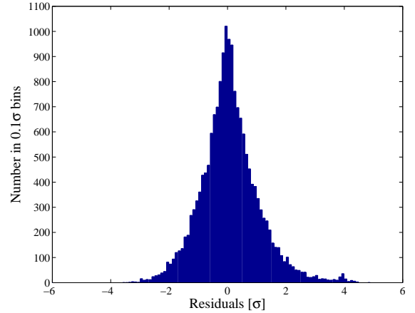
FIG. 3.— The distribution of flux residuals in \sigma units, at all the epochs and at 16 random positions around the position of PTF 12cxj, on the same host galaxy.
