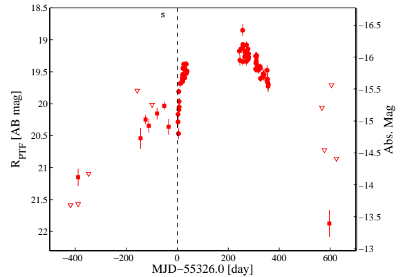
FIG. 7.— The light curve of PTF 10bjb exhibits a clear outburst lasting for \sim 4 months prior to the explosion (identified by the fast rise in the light curve). An additional possible detection is seen \sim 400 days prior to the explosion, but we do not consider it to be a good candidate since it is based on a single binned detection (see the discussion about false-alarm probability in §4.2). The upper limits corresponds to 5\sigma bounds calculated in 15-day bins.
