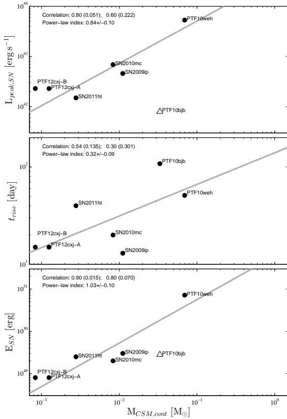
FIG. 20.— Like Figure 19, but with the CSM mass estimated based on Equation 5.
